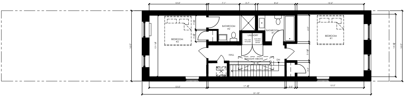
1318 MADISON AVE. THIRD FLOOR 829 G.S.F.
