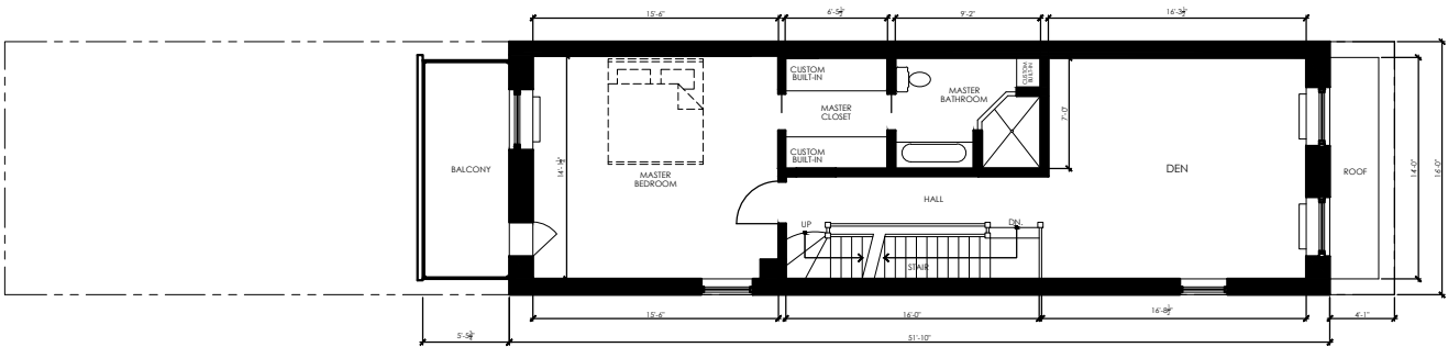
1318 MADISON AVE. SECOND FLOOR 829 G.S.F.
