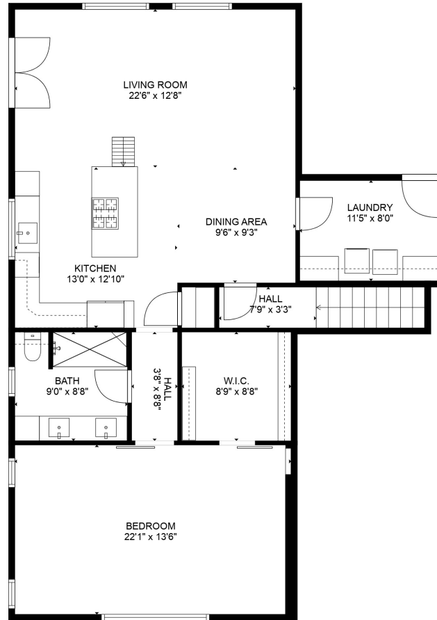
FLOOR 2
