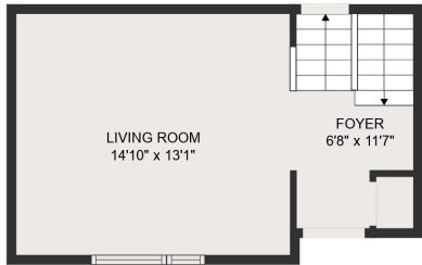
FLOOR 2
