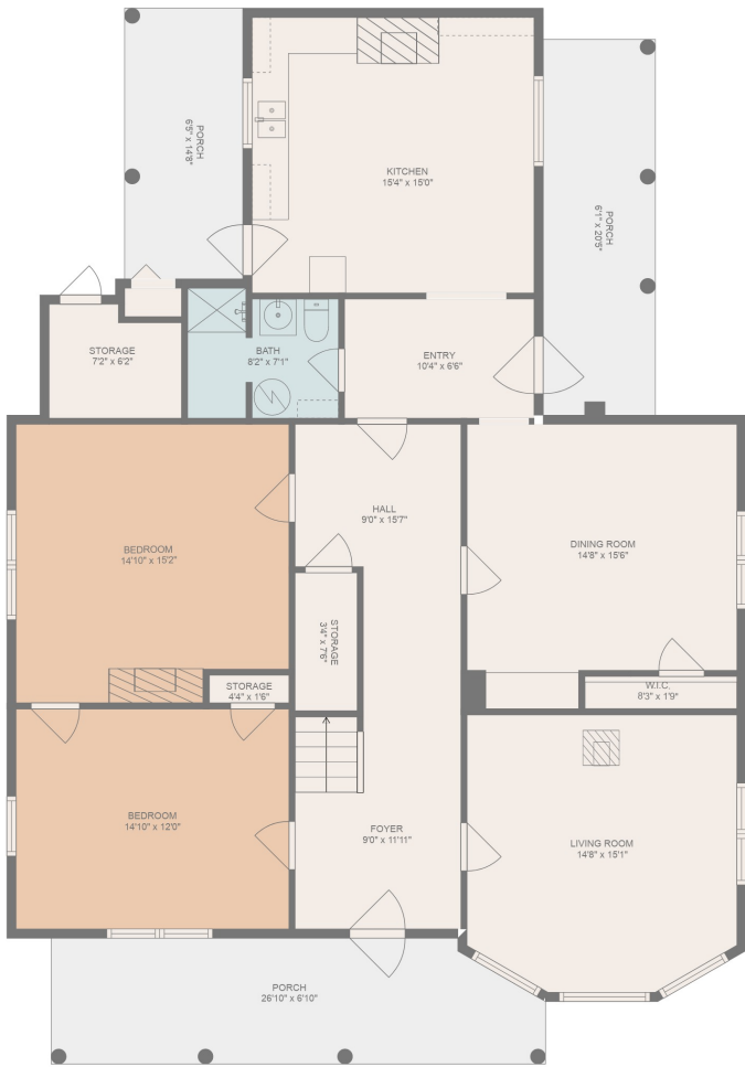
FLOOR 1
