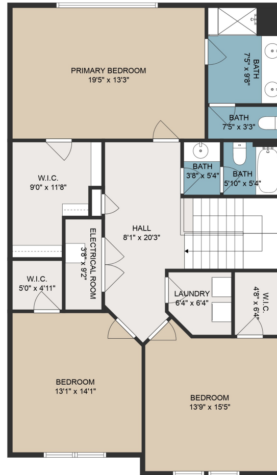
FLOOR 2
