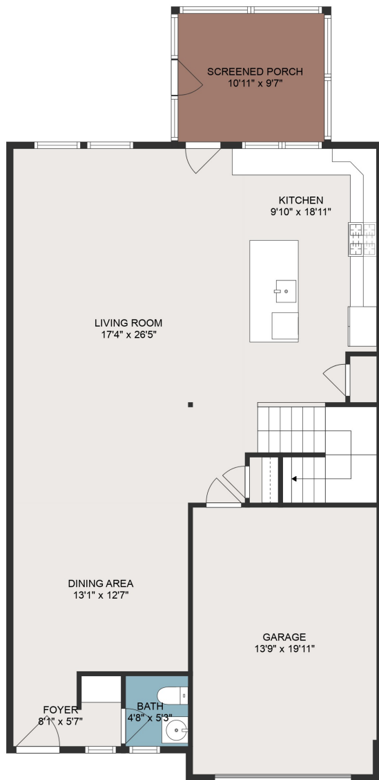
FLOOR 1
