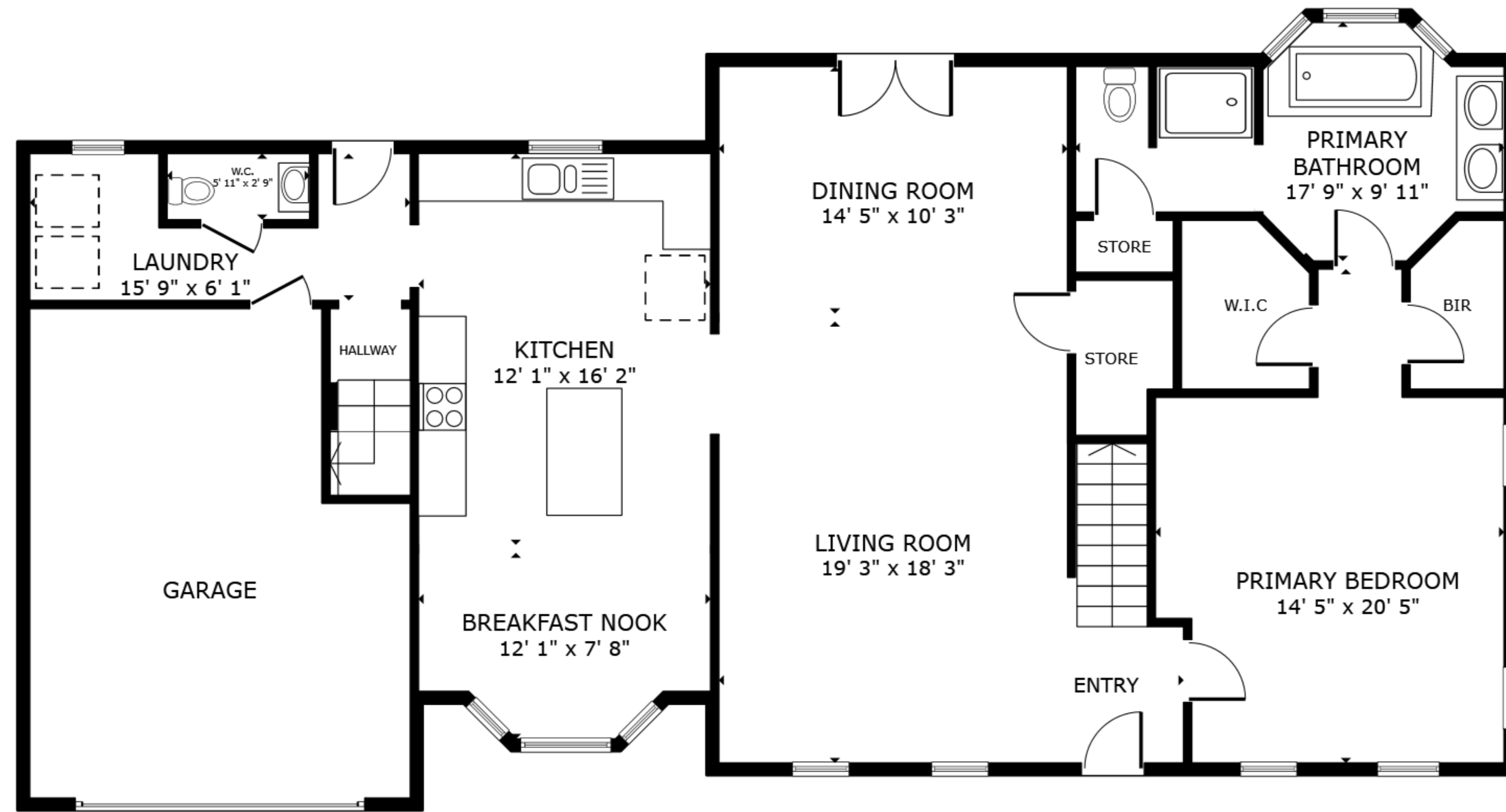
FLOOR 1
