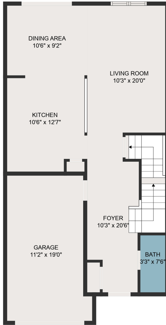
FLOOR 2
