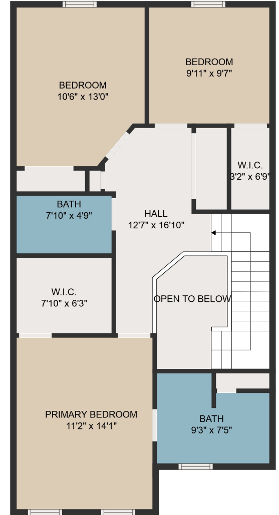
FLOOR 3
