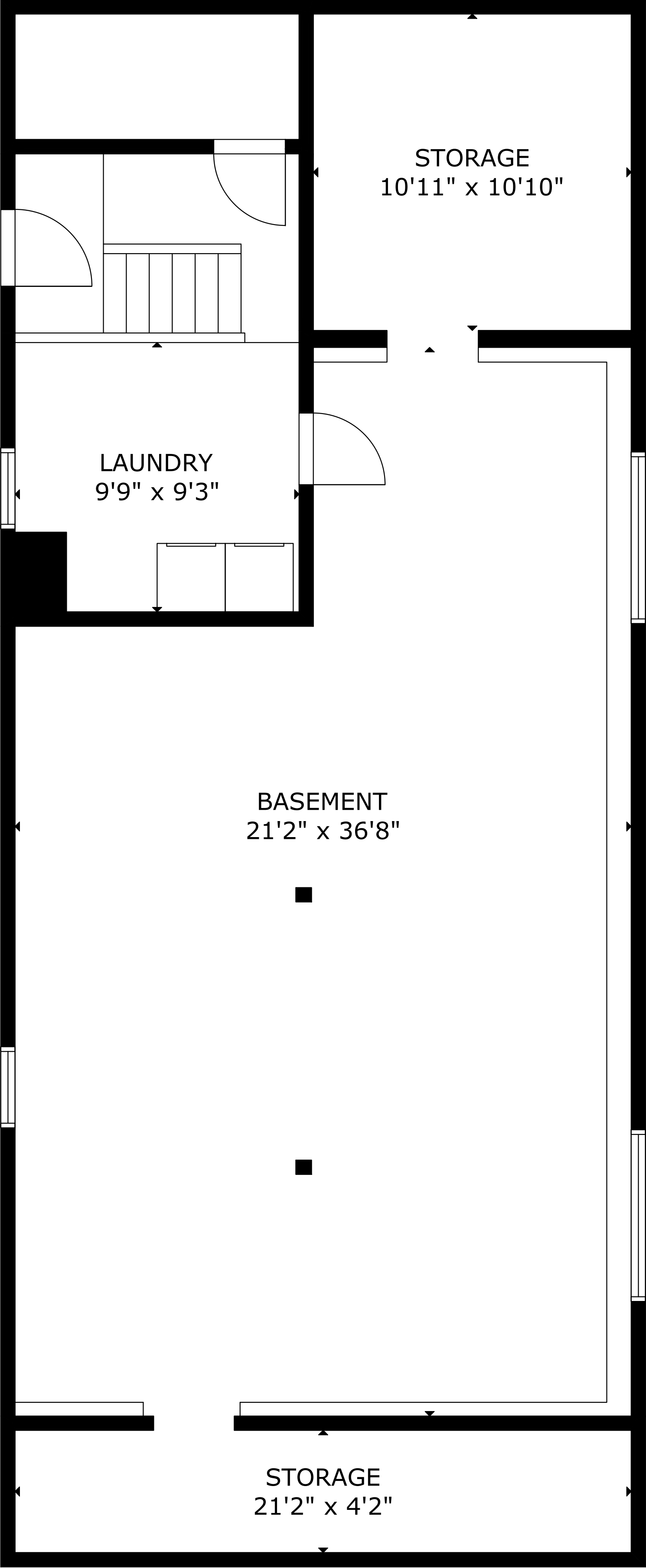
LOWER LEVEL
