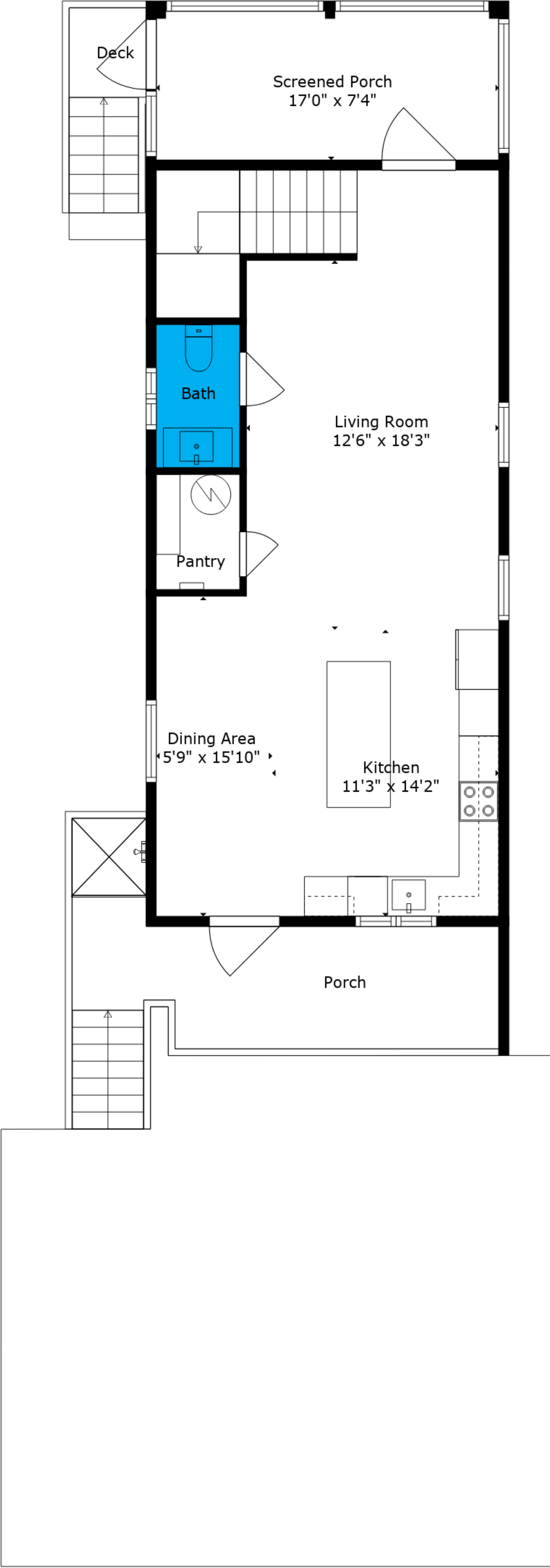
Floor 1
