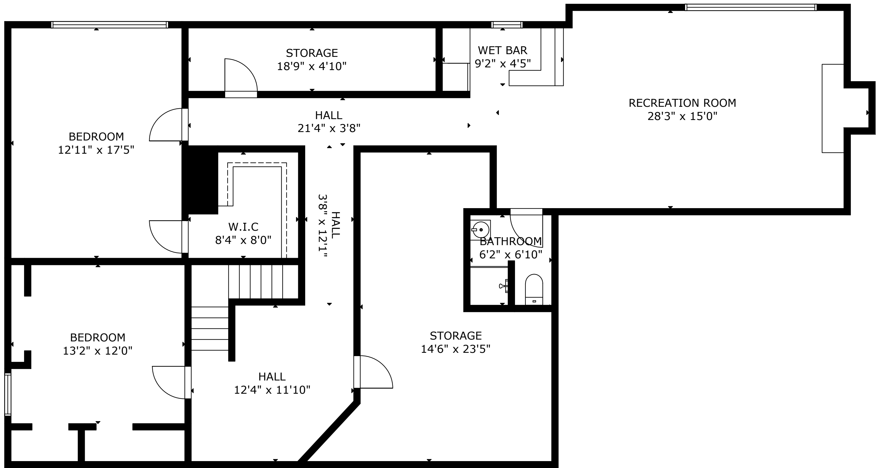
LOWER LEVEL
