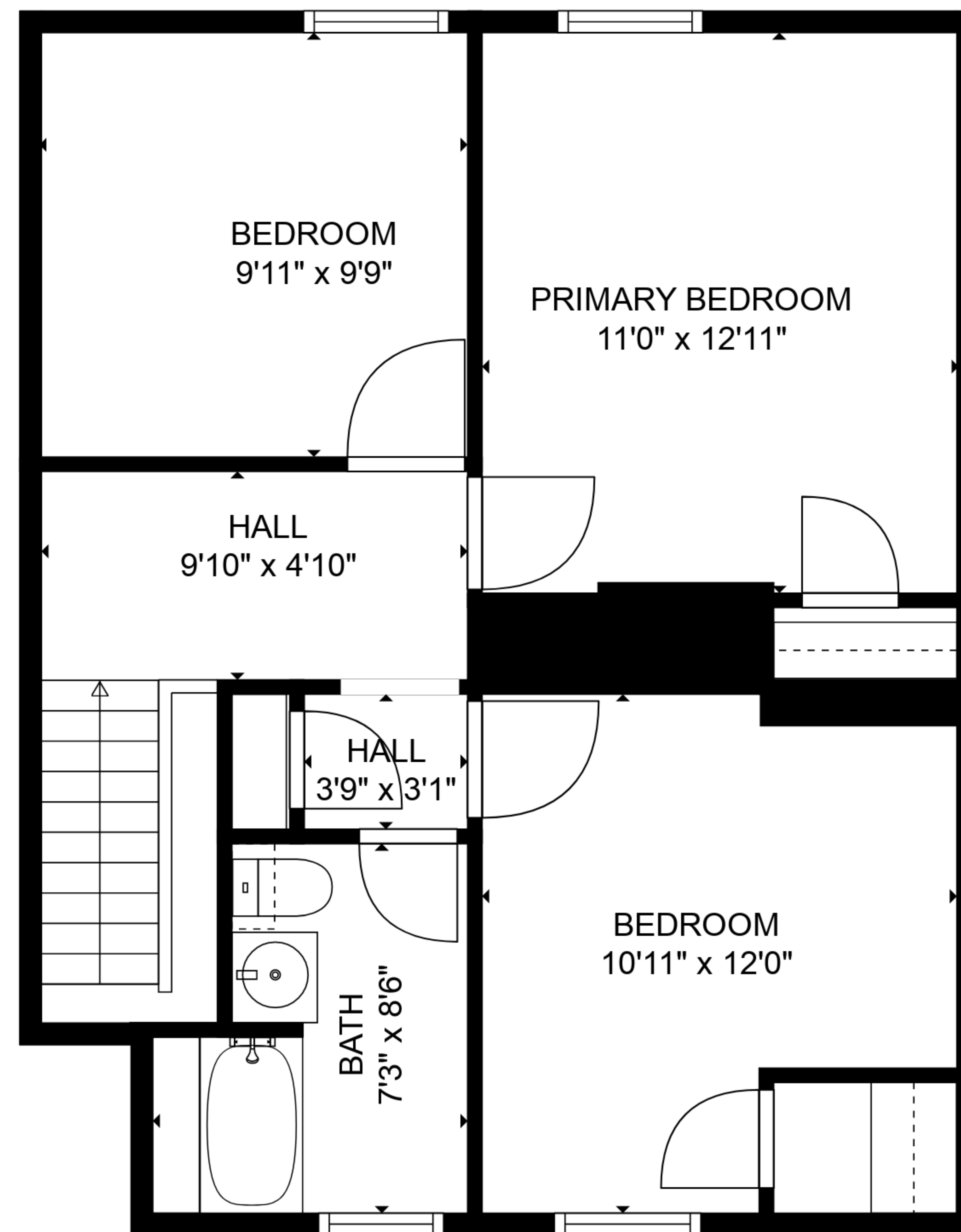
FLOOR 2
