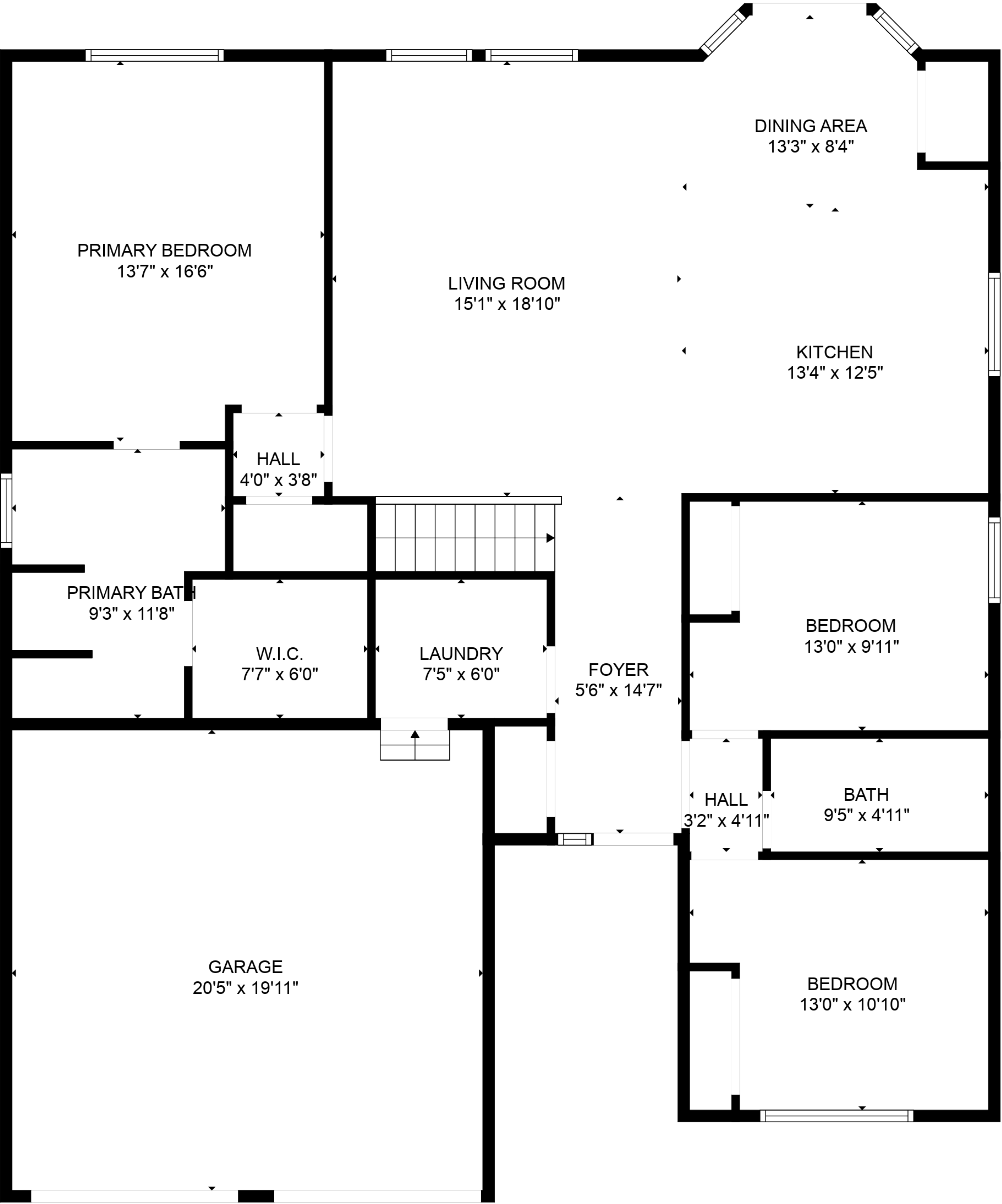
FLOOR 2
