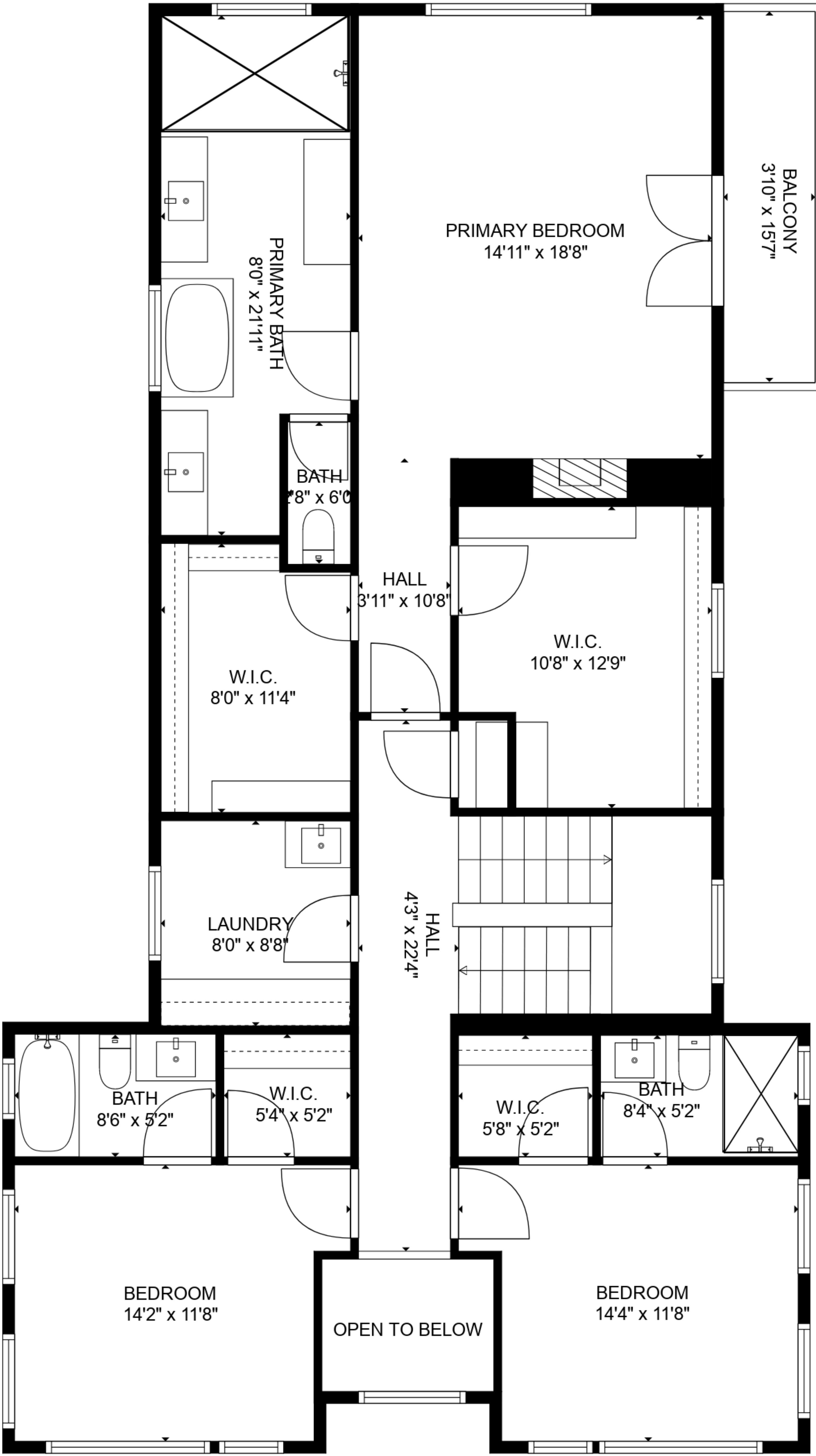
FLOOR 2
