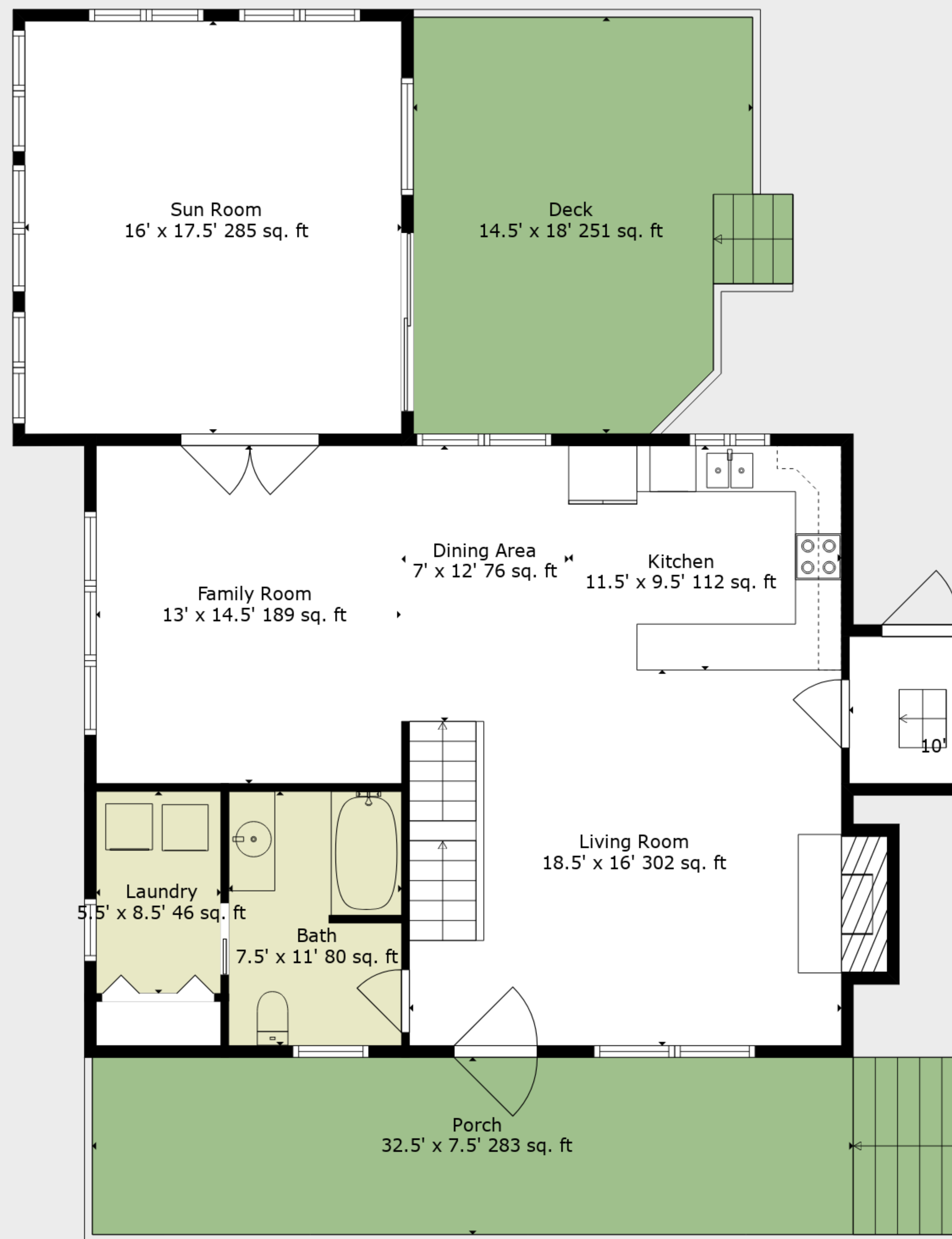
Floor 2
