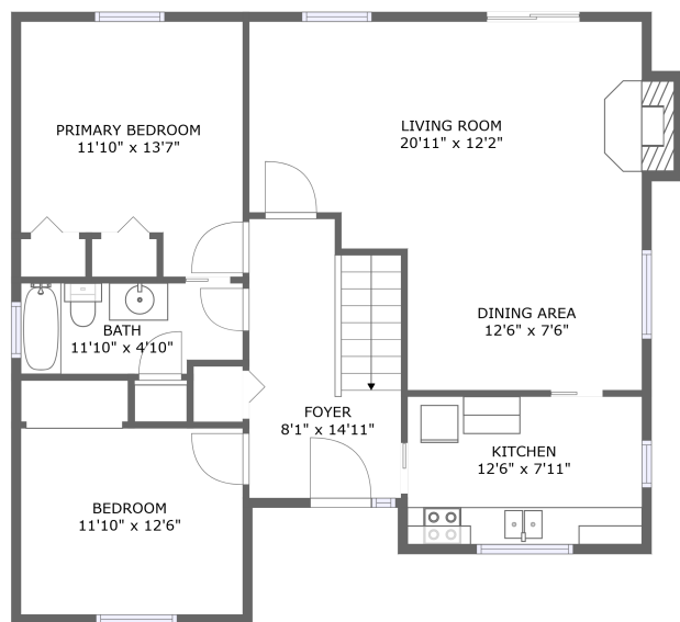
FLOOR 2
