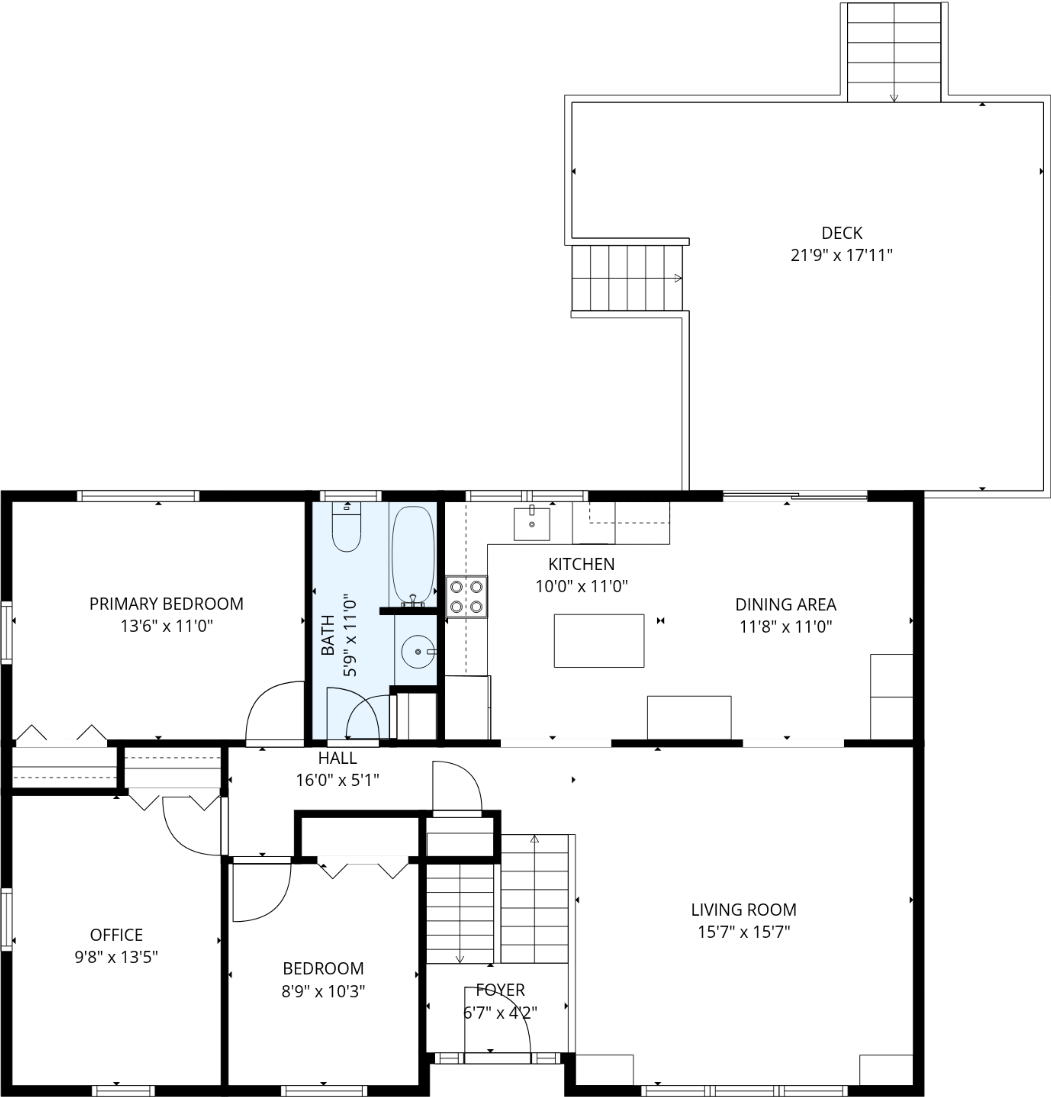
2nd floor
