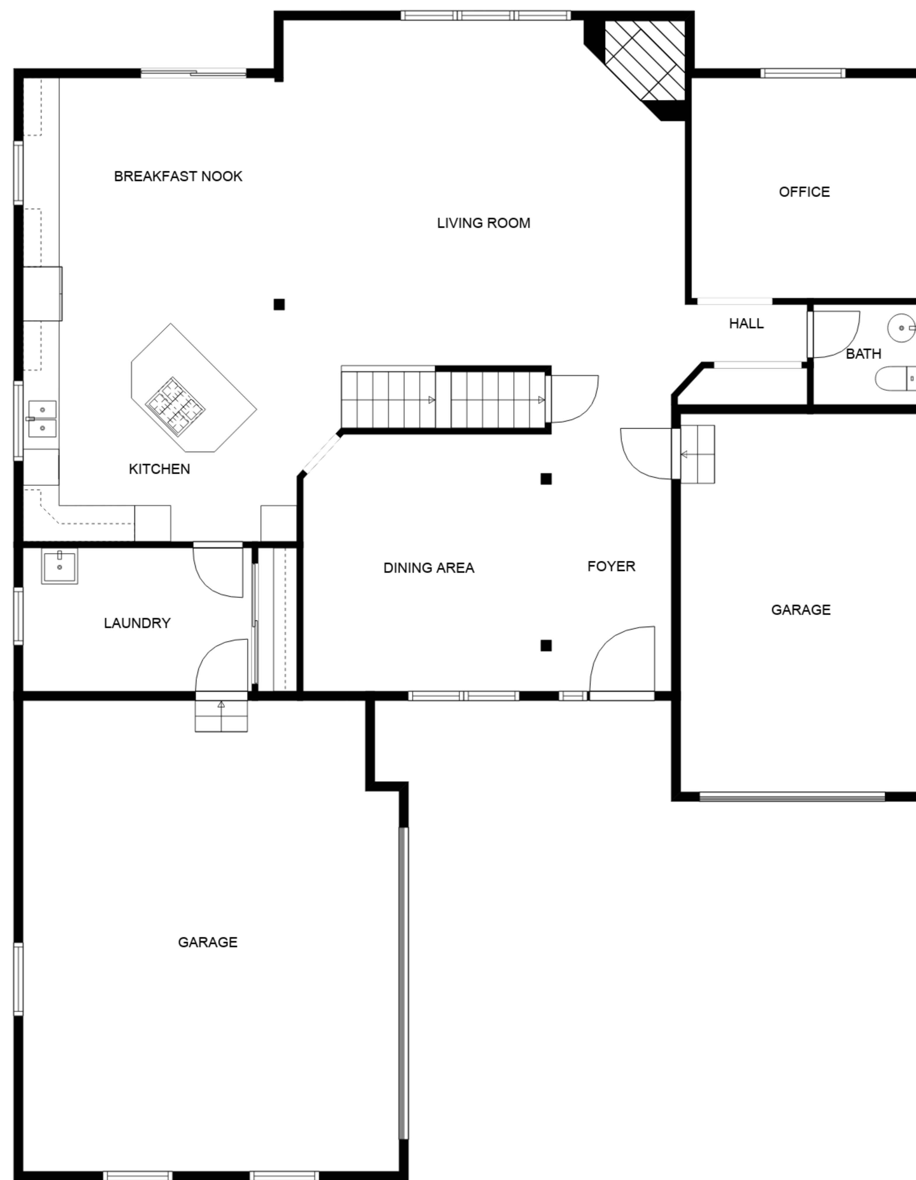
FLOOR 2
