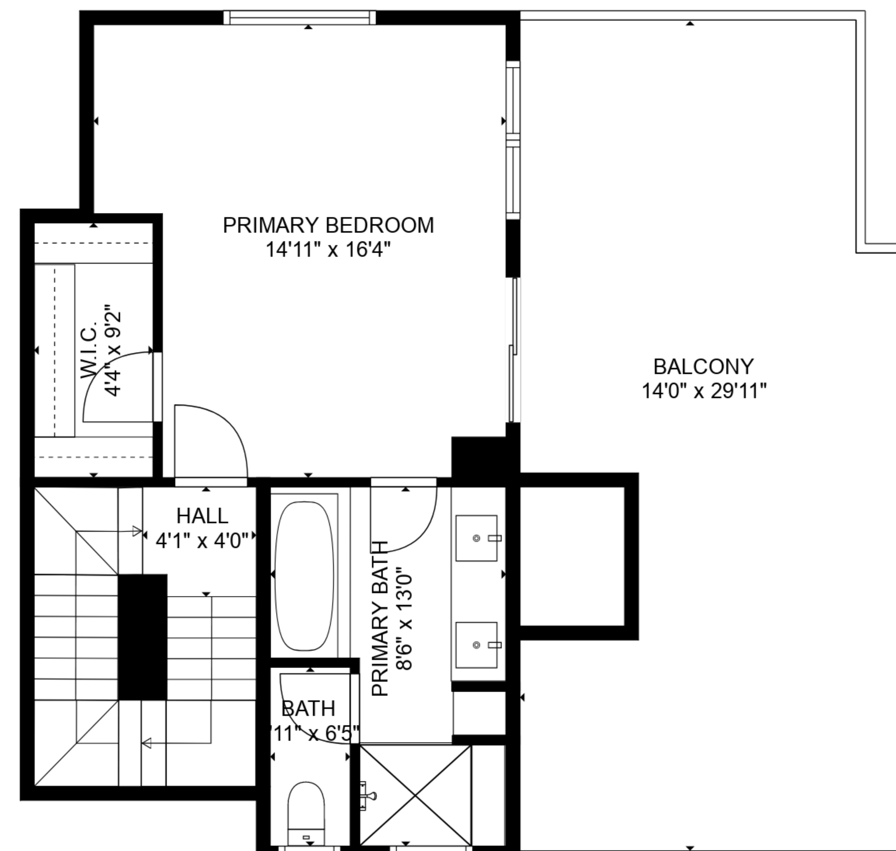
FLOOR 3
