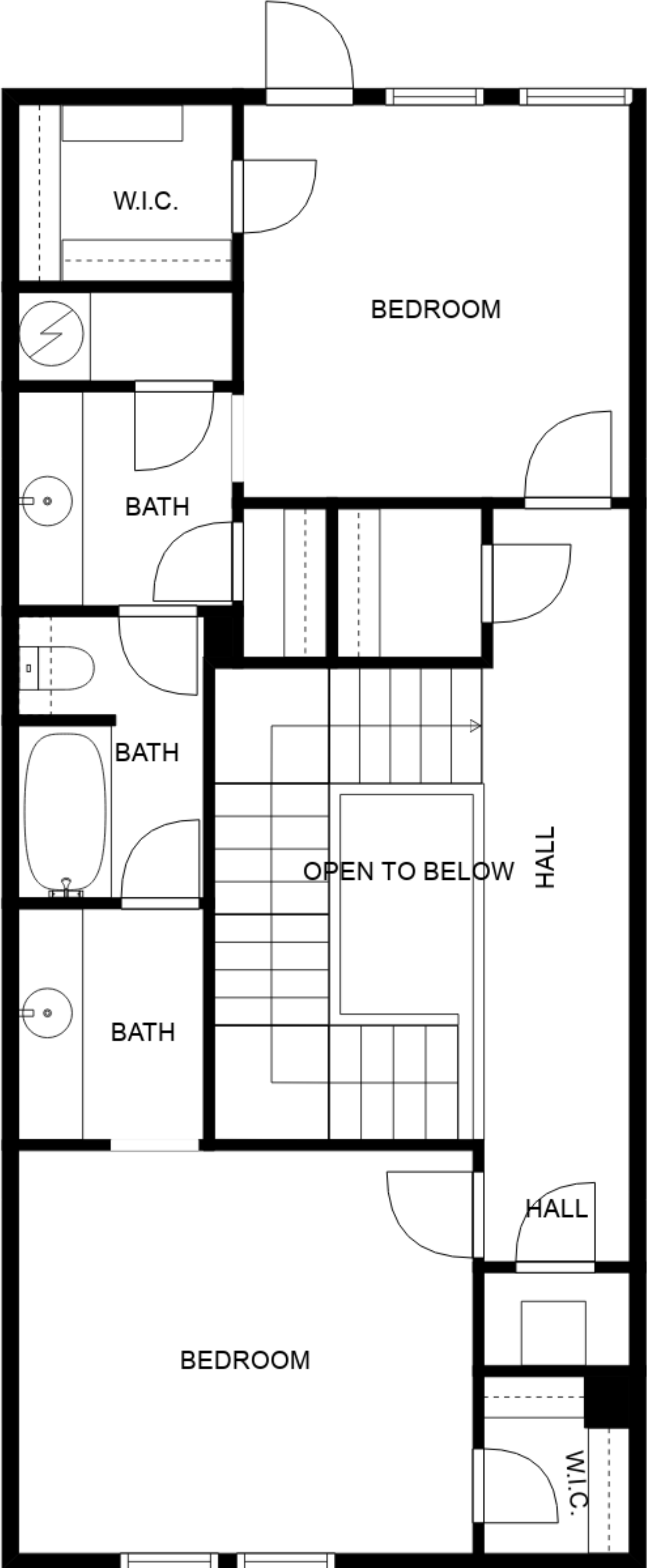
FLOOR 3
