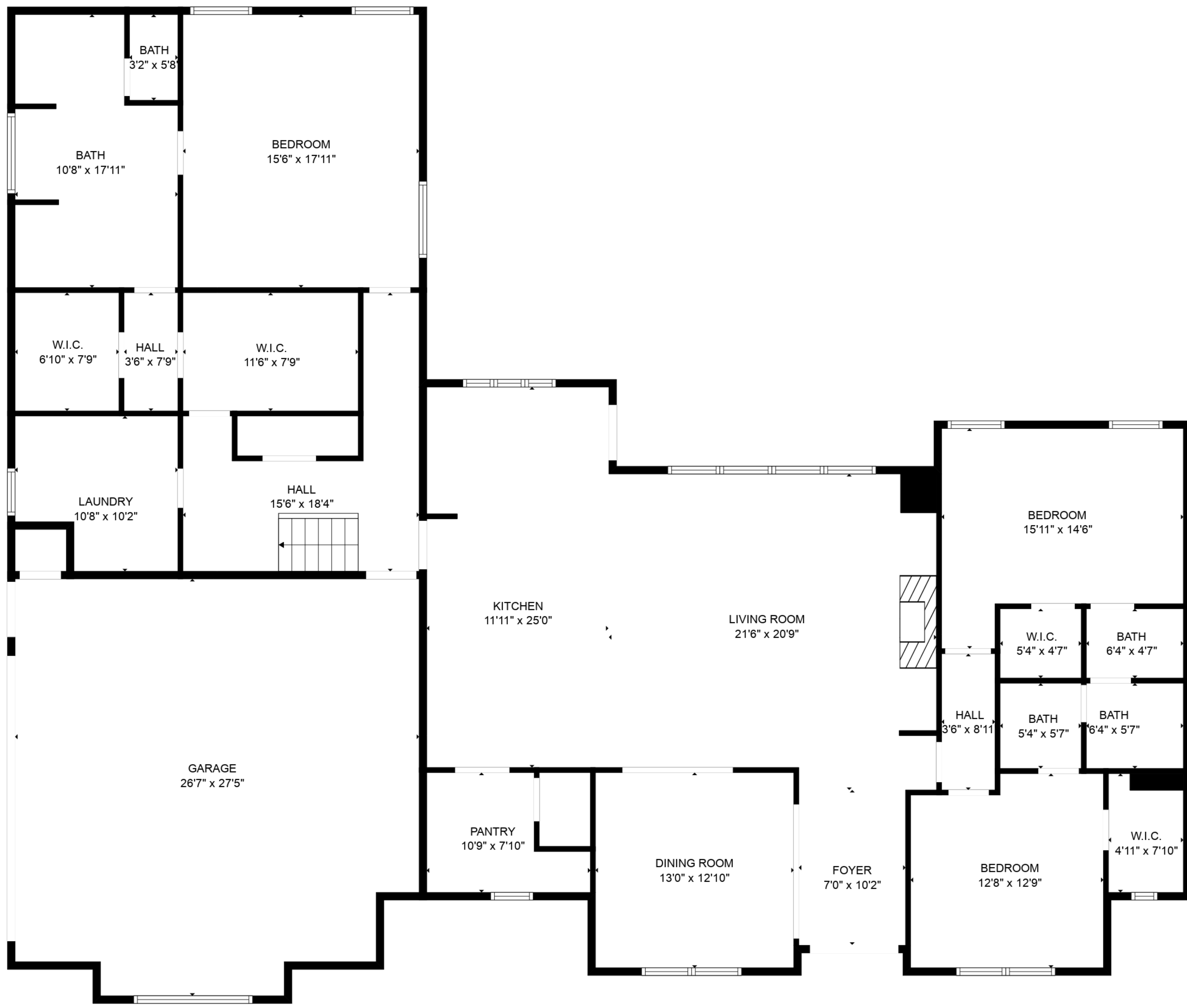
FLOOR 1
