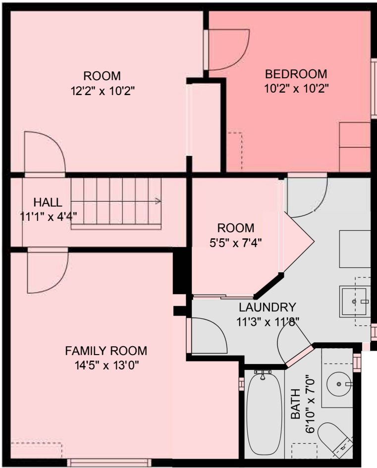
FLOOR 1
