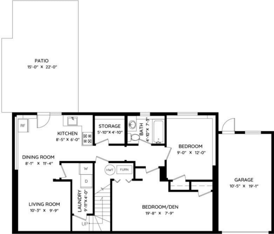
LOWER FLOOR 966 SQ.FT. CH: 8'-0"
