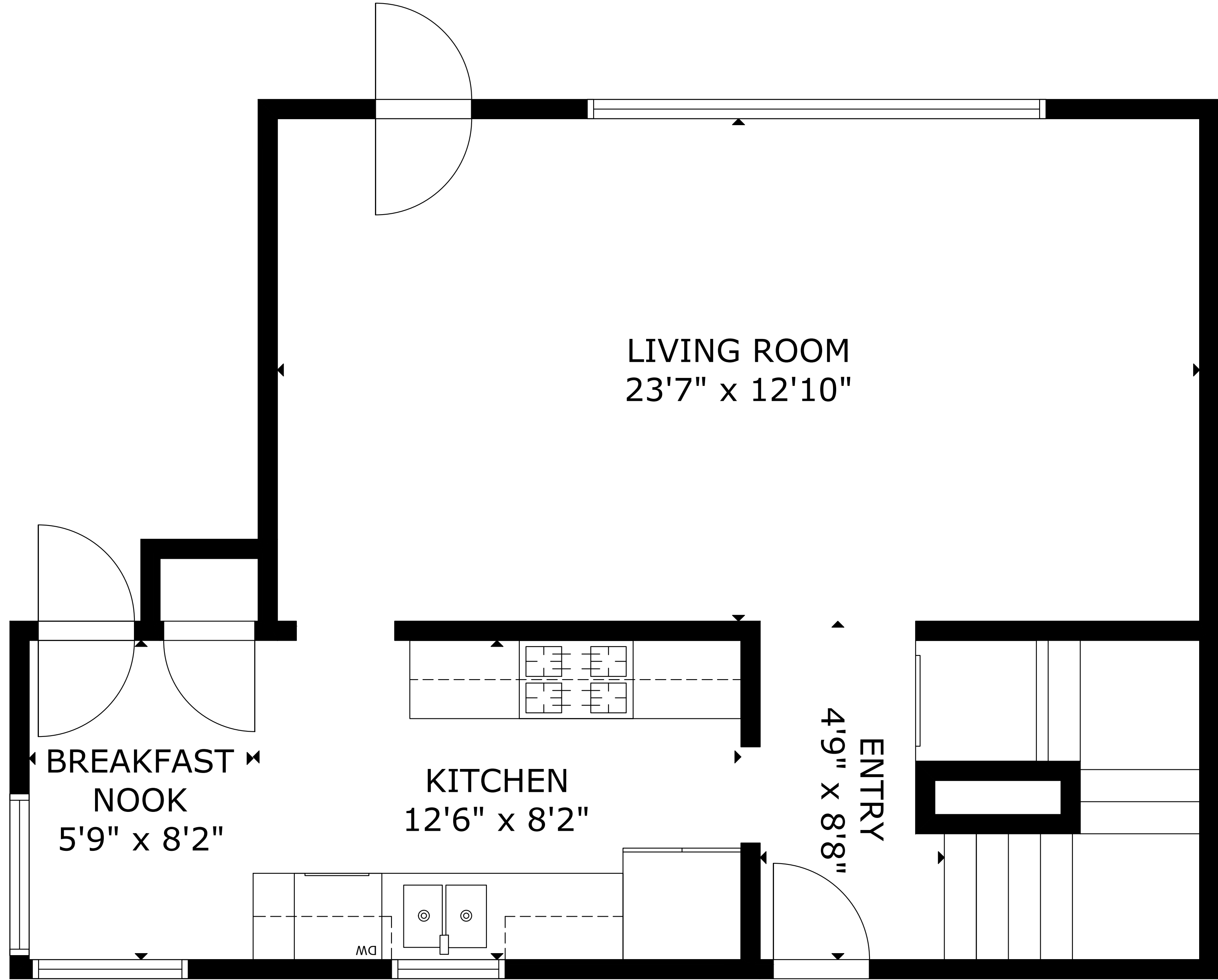
FLOOR 1
