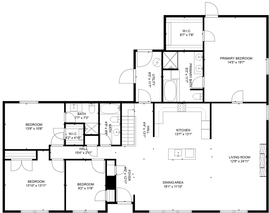
FLOOR 2
