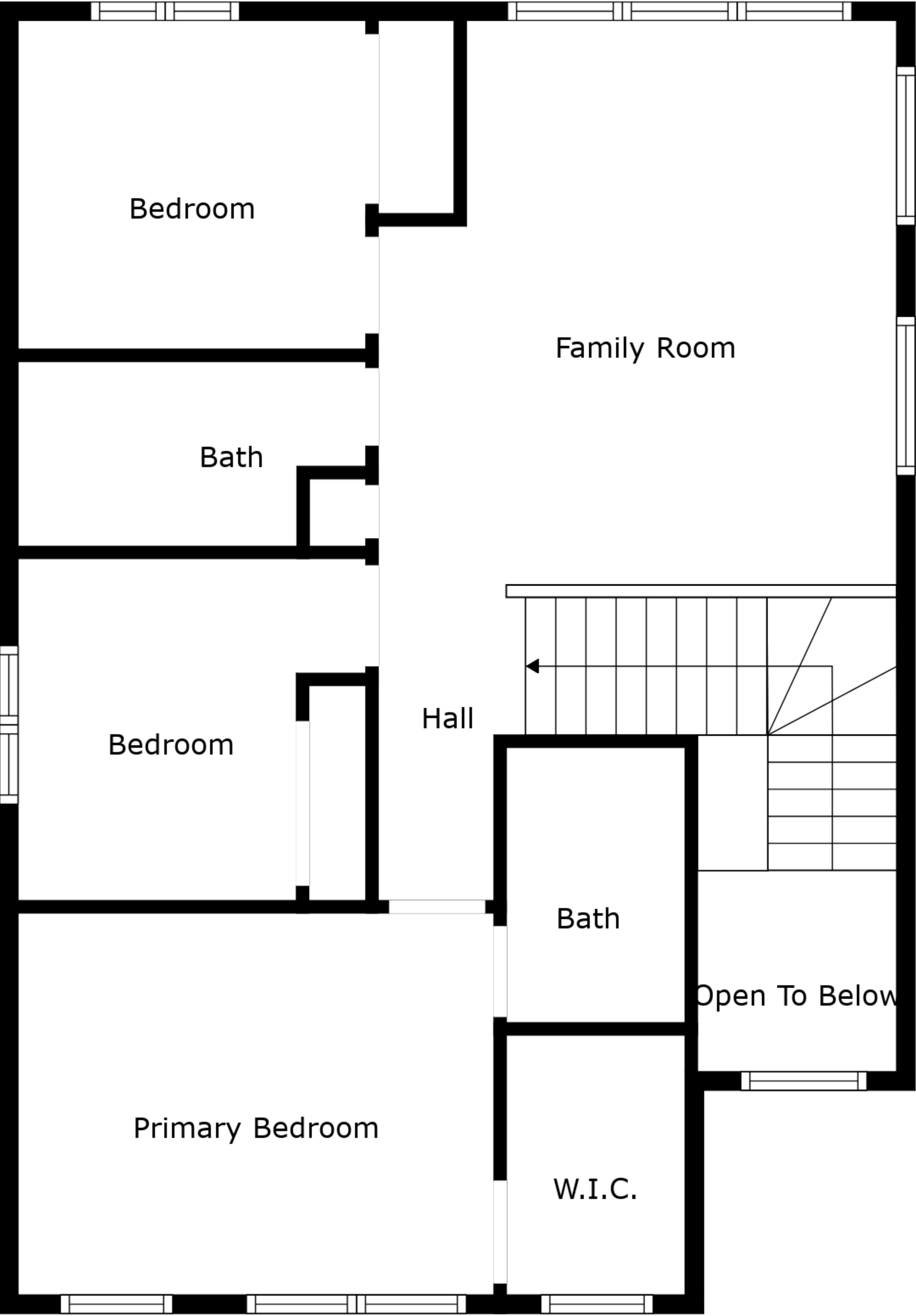
Floor 3
