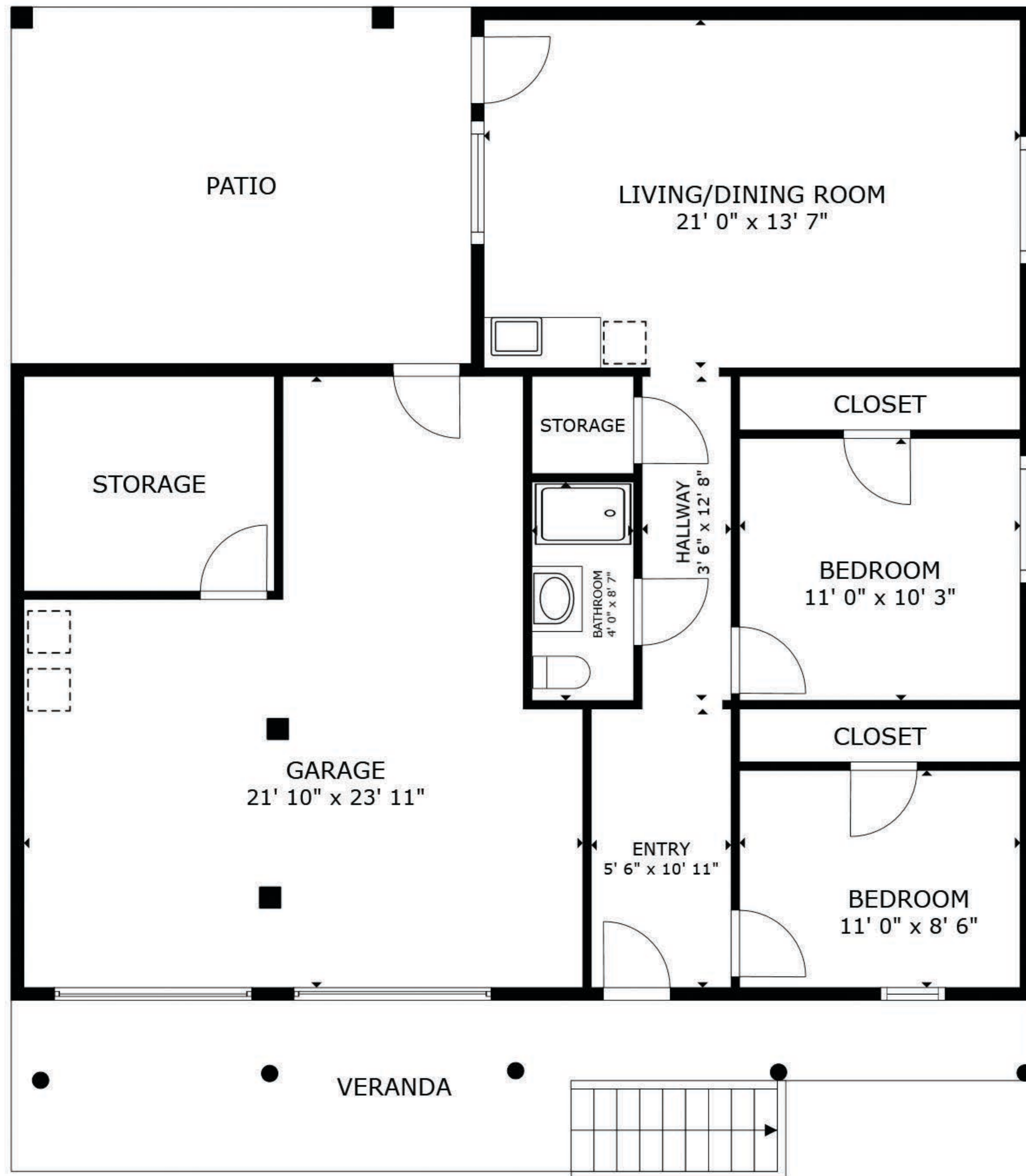
FLOOR 1
