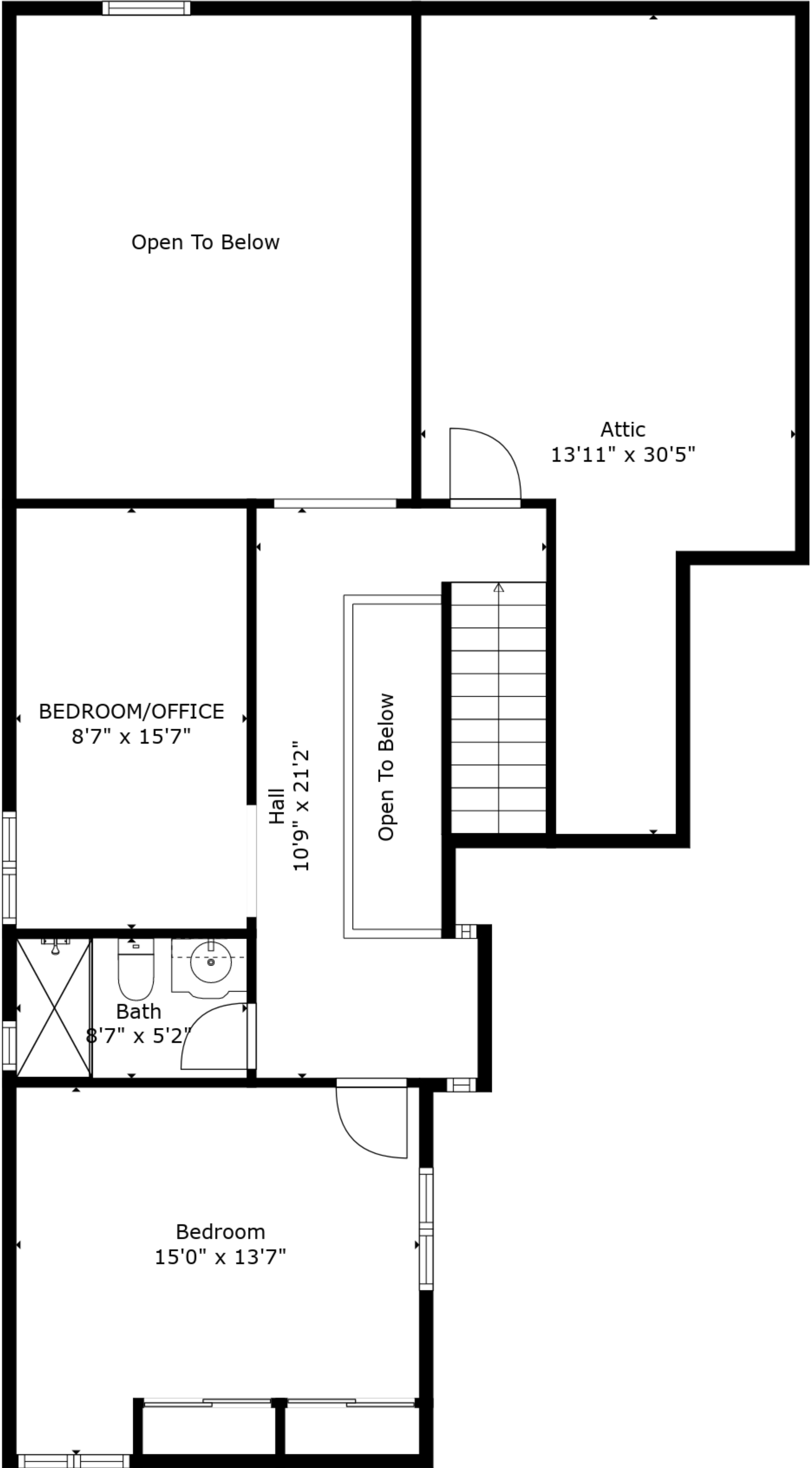
Second Floor
