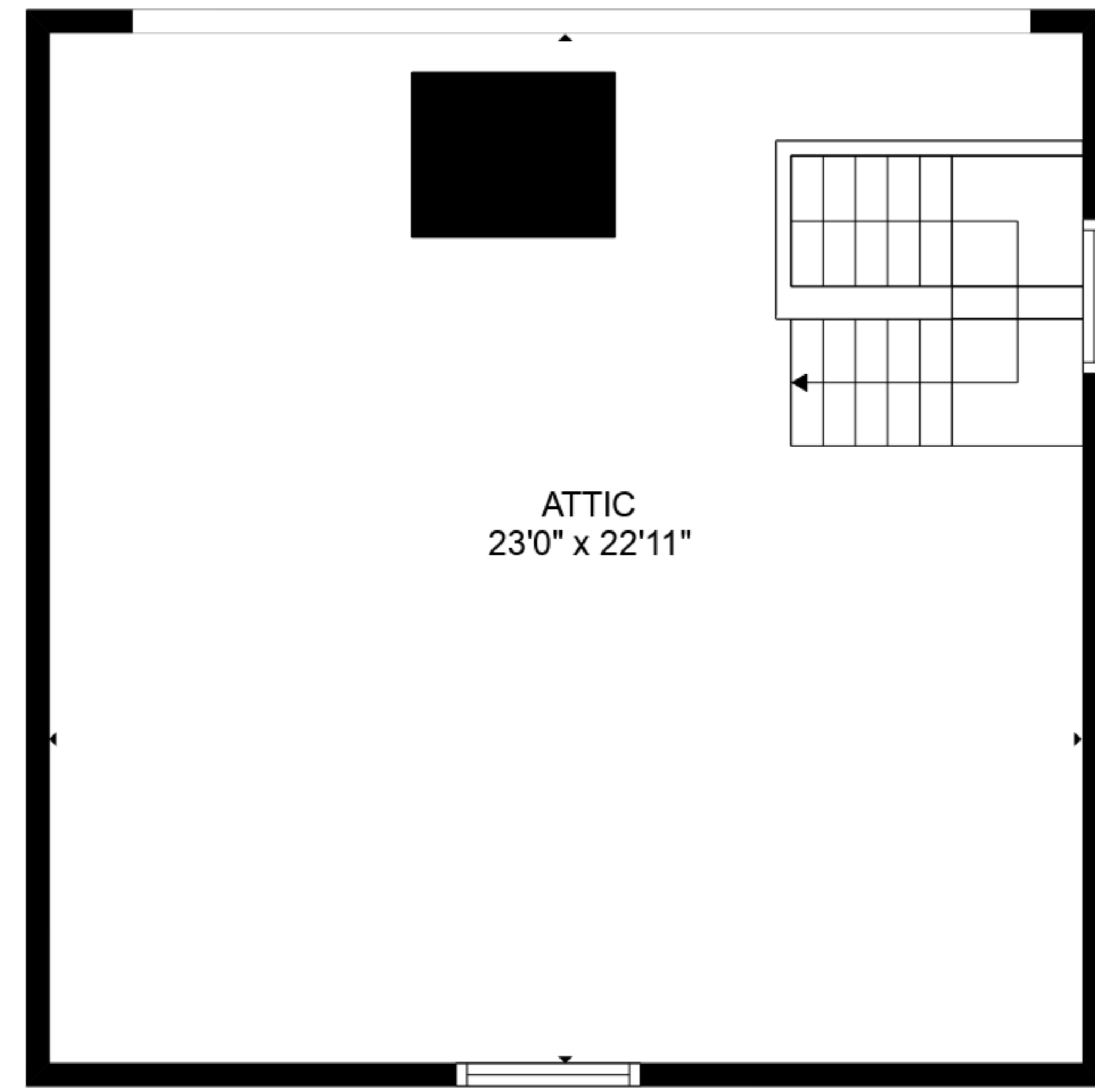
FLOOR 4
