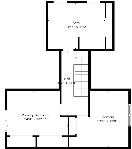
Floor 3
