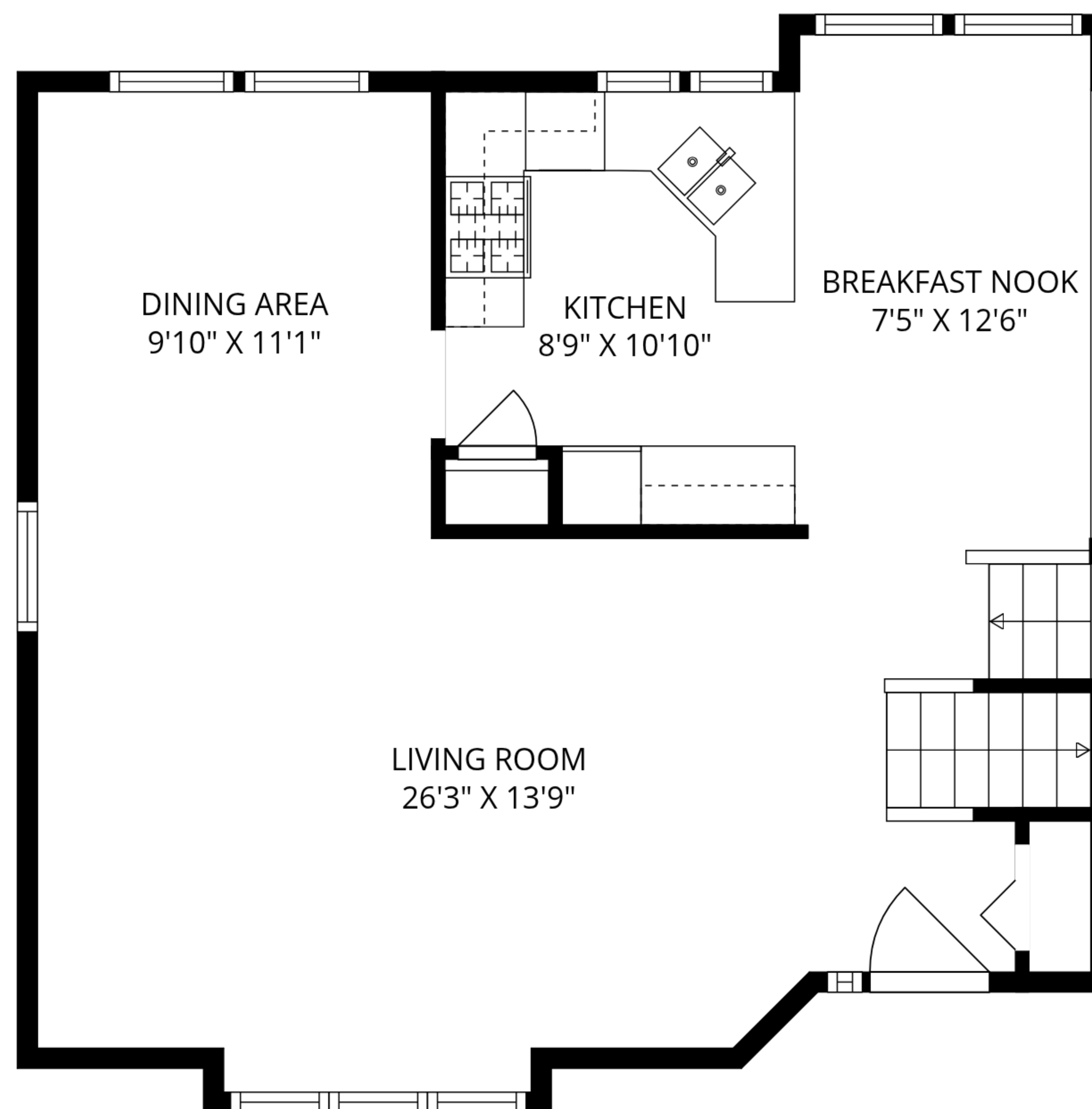
1ST FLOOR
