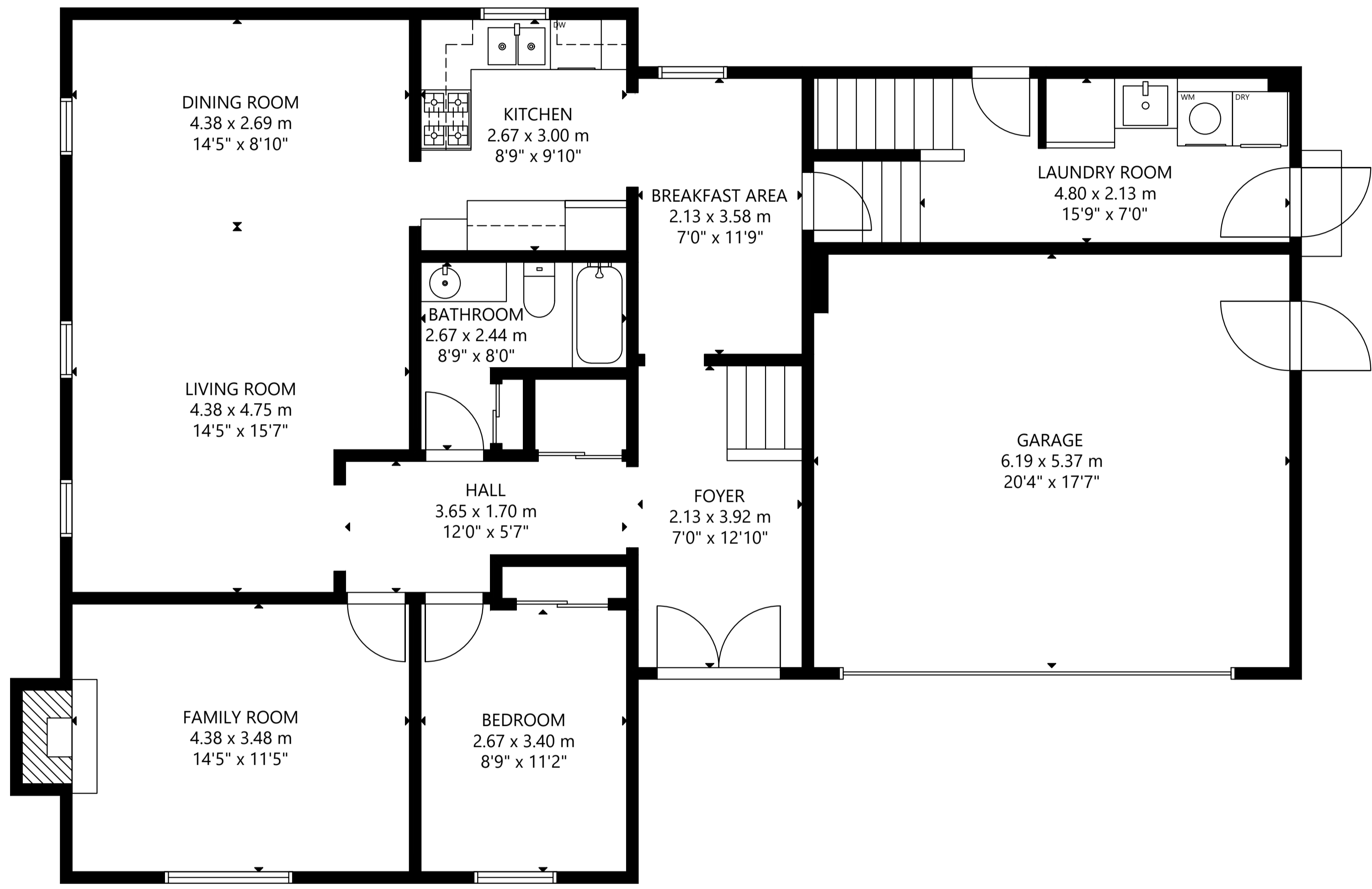
MAIN FLOOR
