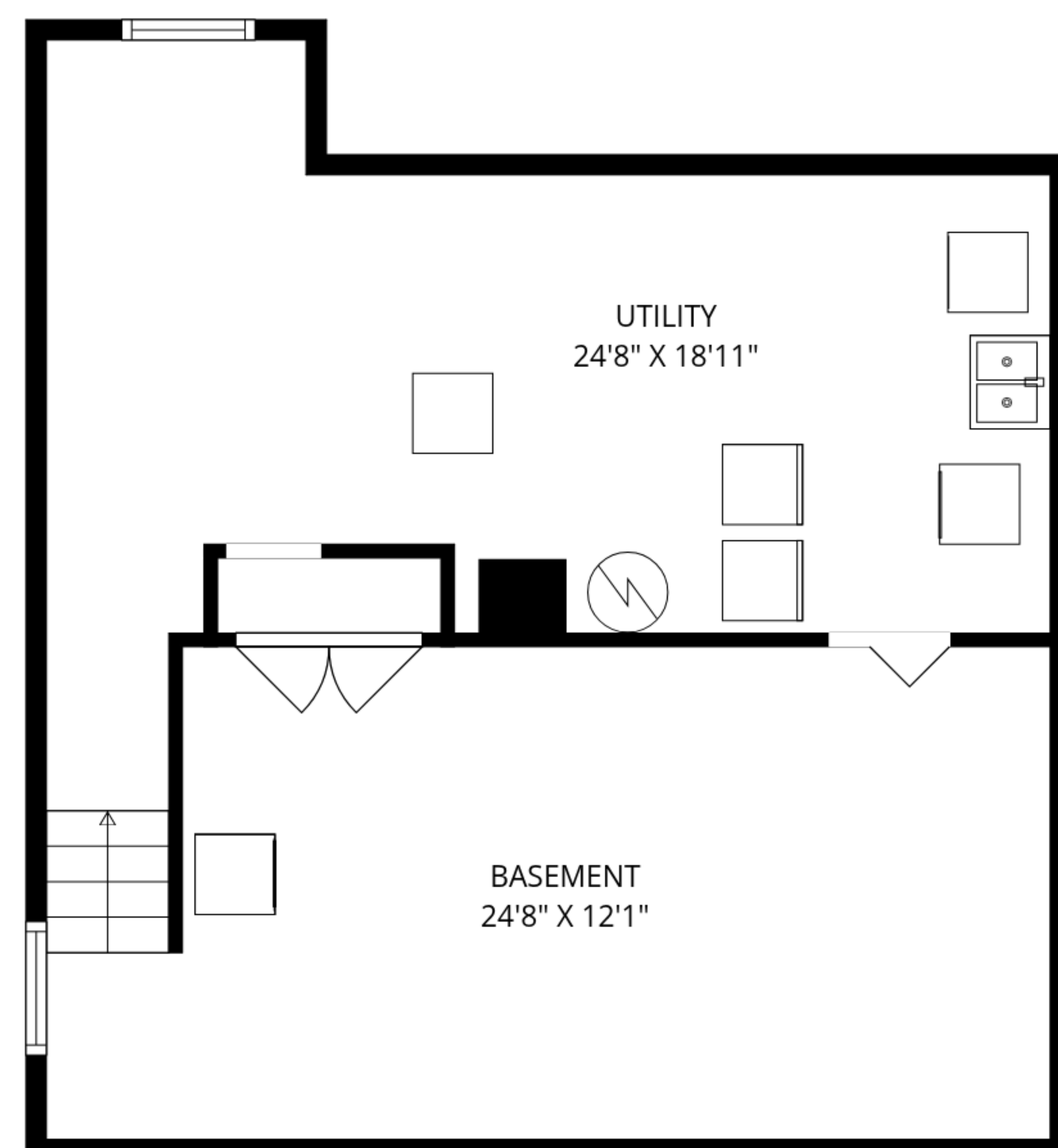
BASEMENT 1
