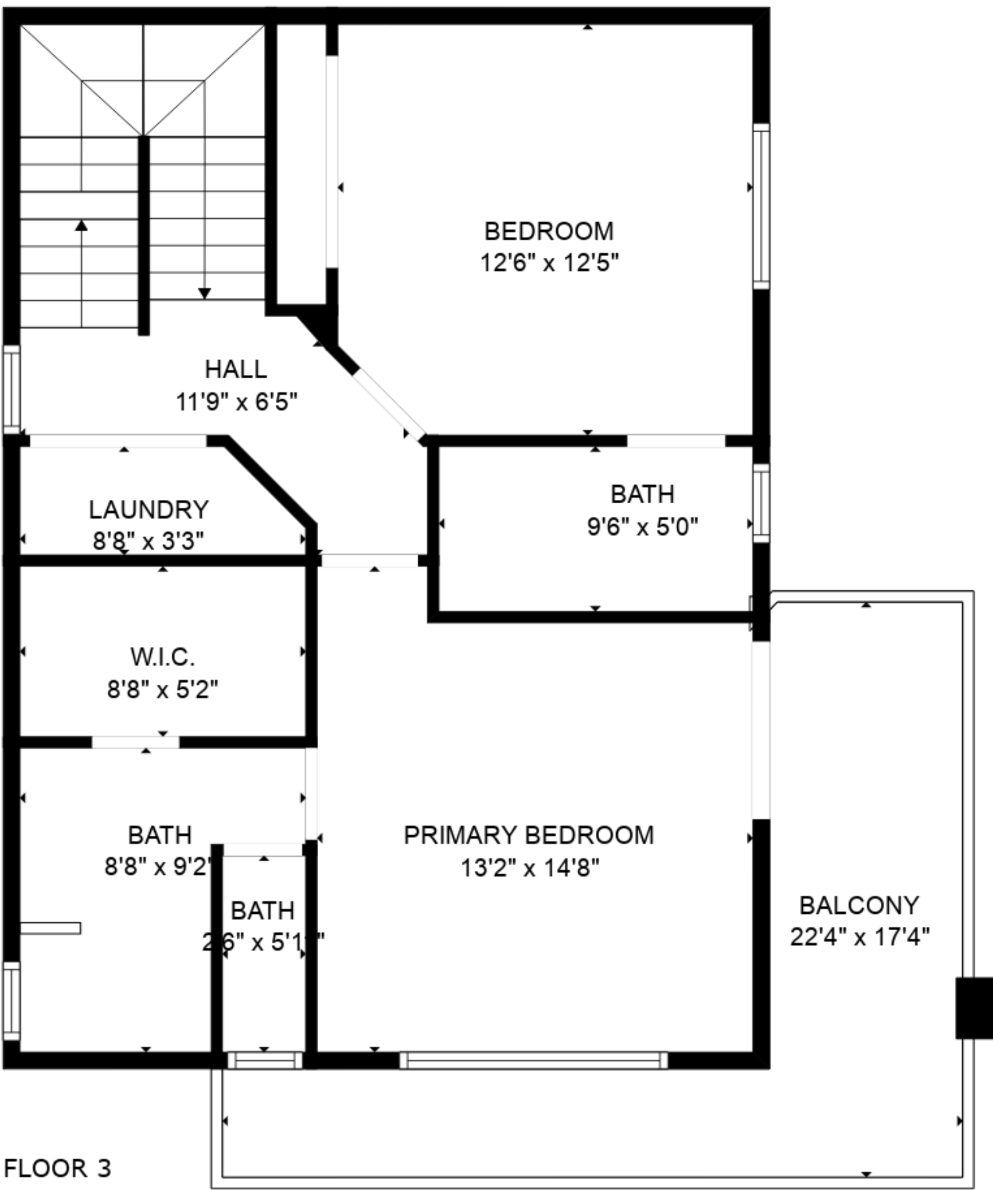
FLOOR 3
