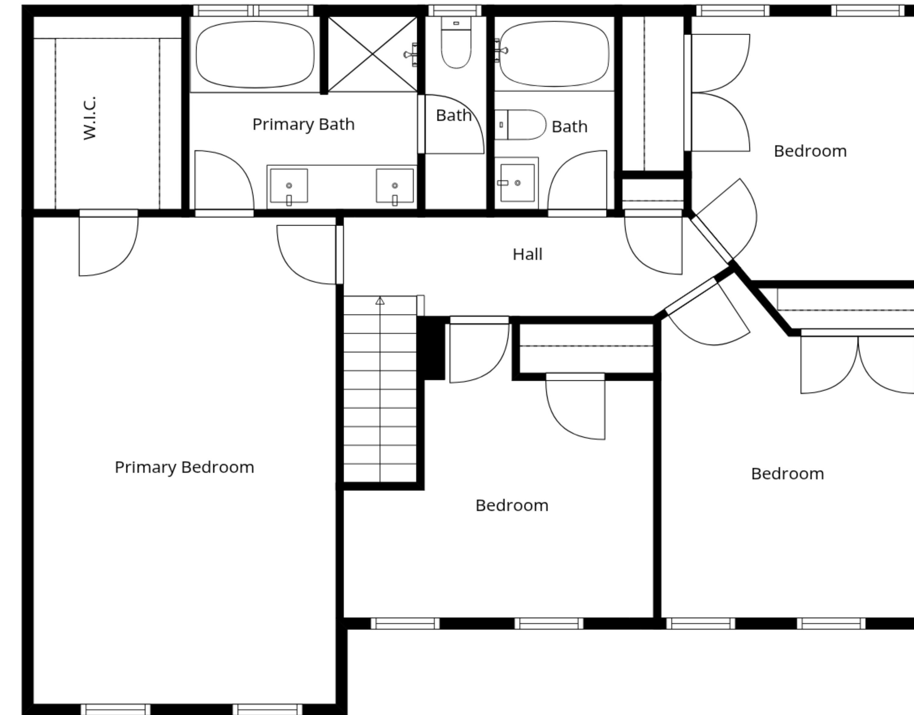
Floor 3
