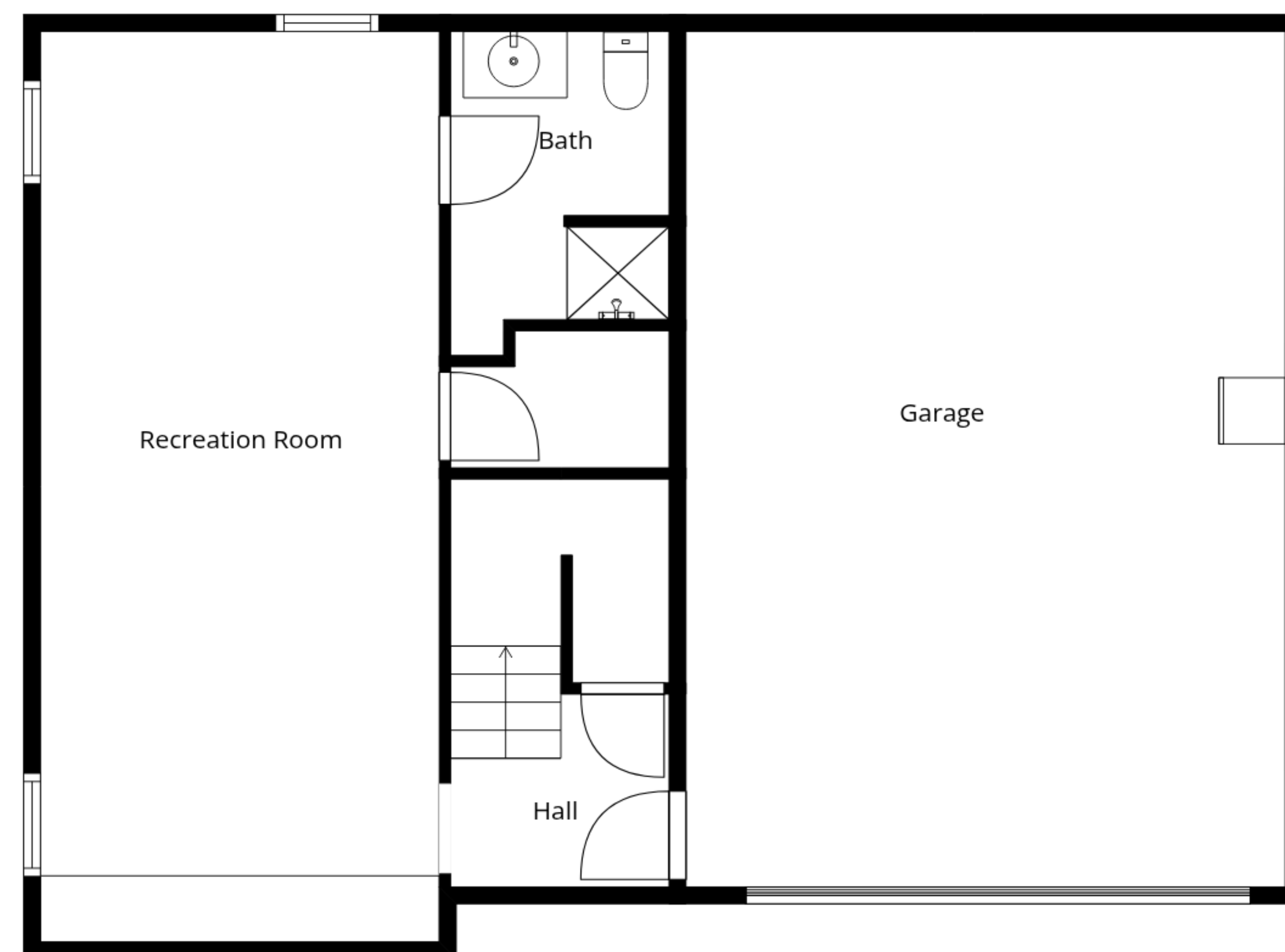
Floor 1
