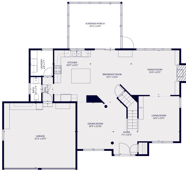
FLOOR 2
