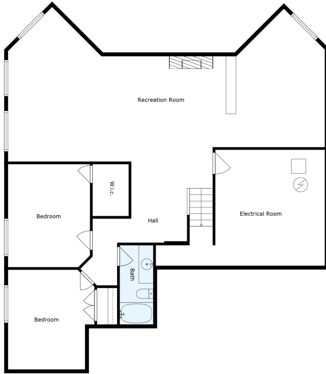
Floor 1
