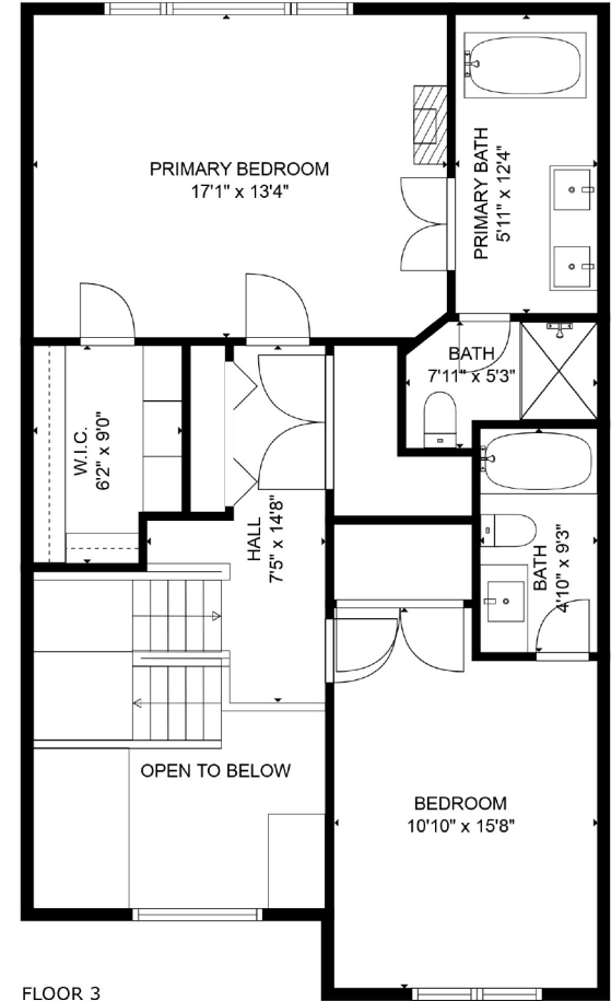
FLOOR 3
