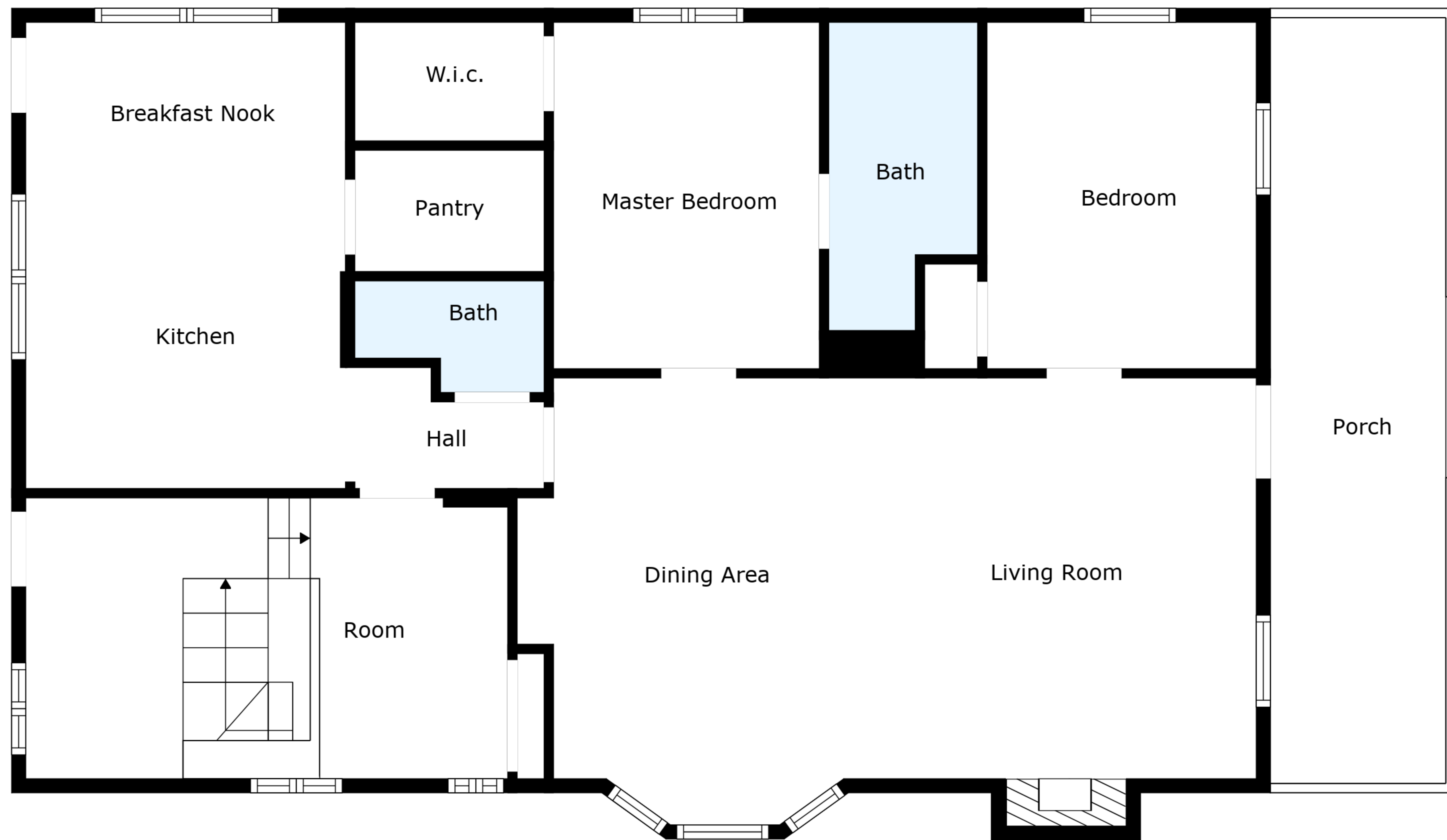
Floor 2
