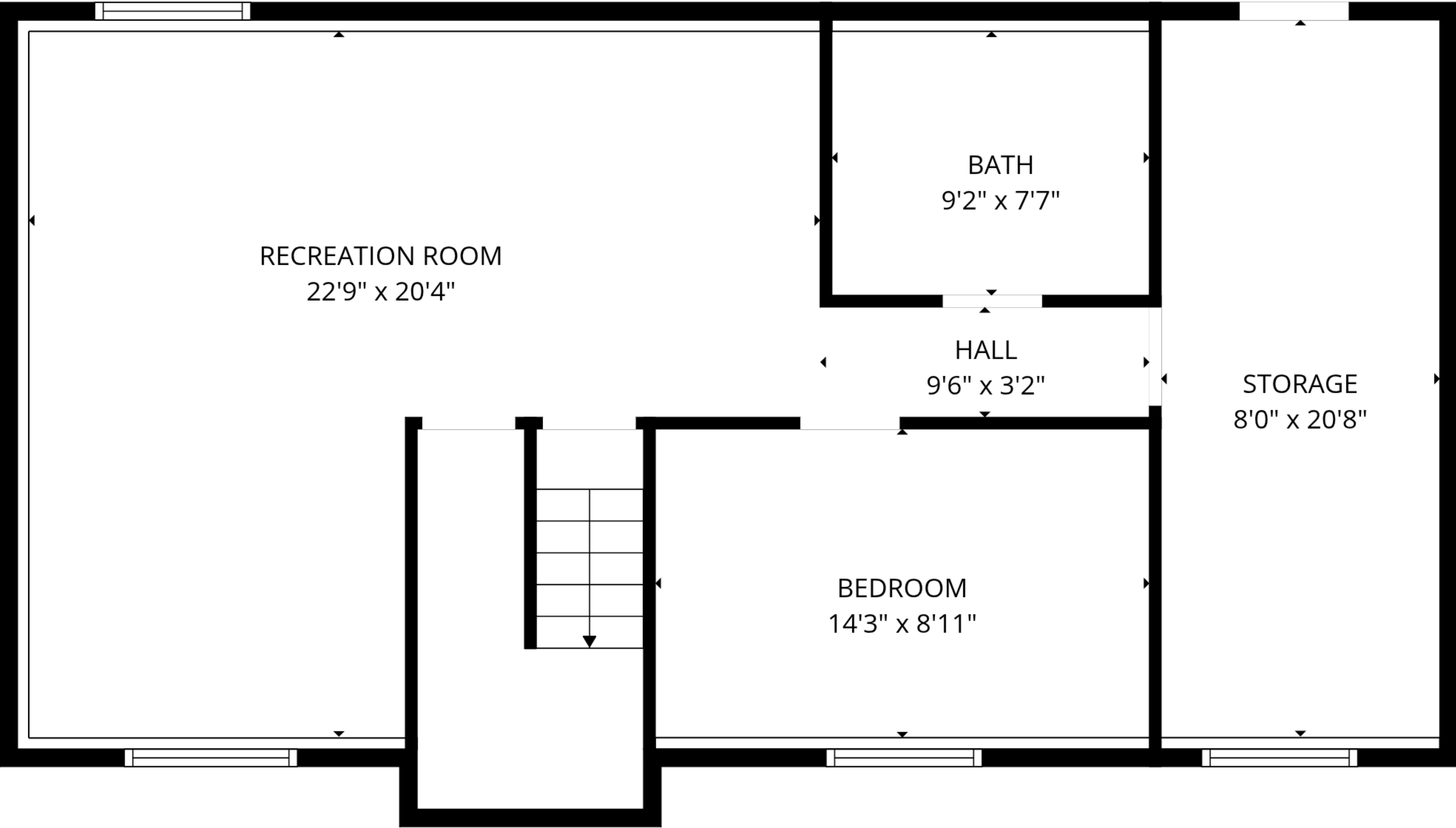
FLOOR 1
