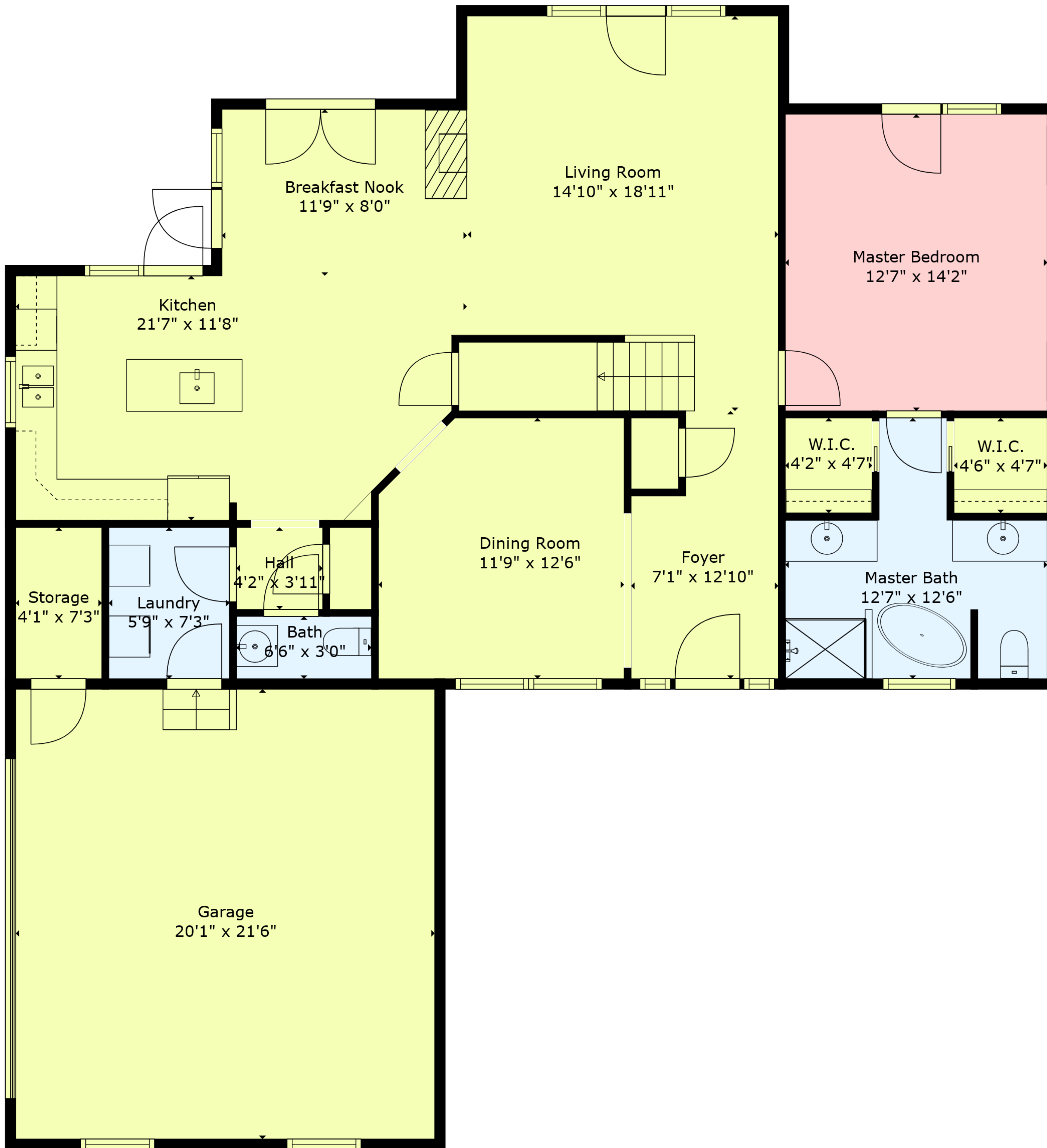
Floor 1
