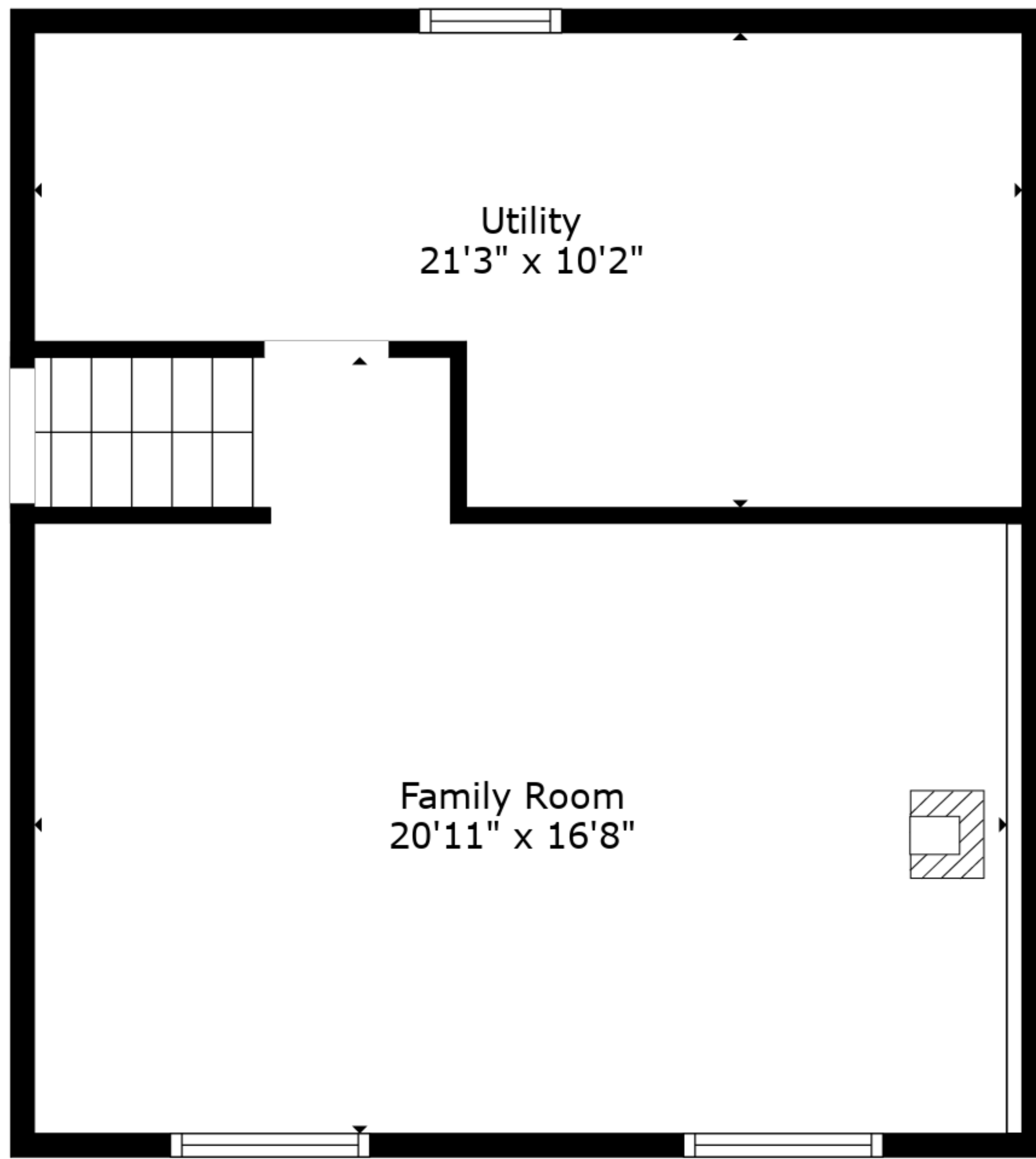
Floor 1
