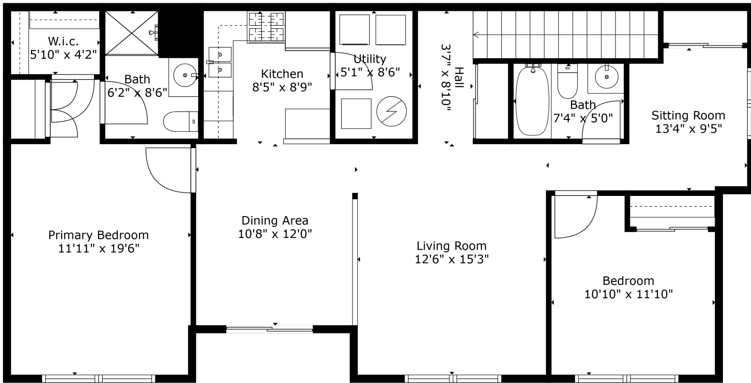
Floor 2
