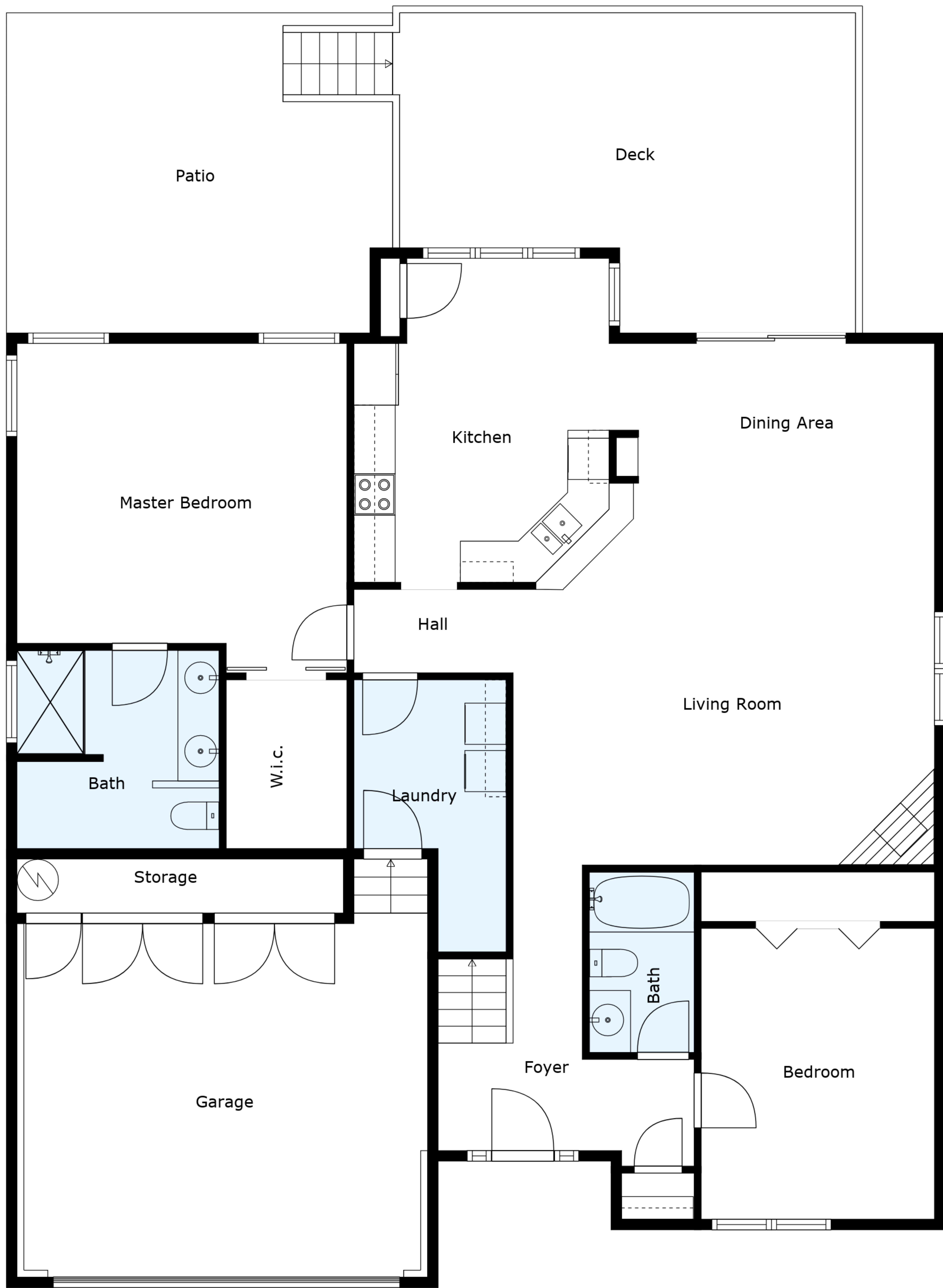
Floor 1
