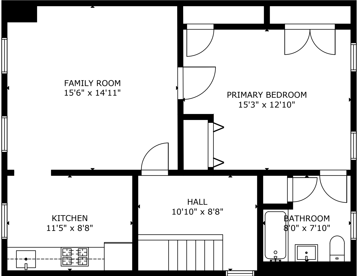
THIRD FLOOR
