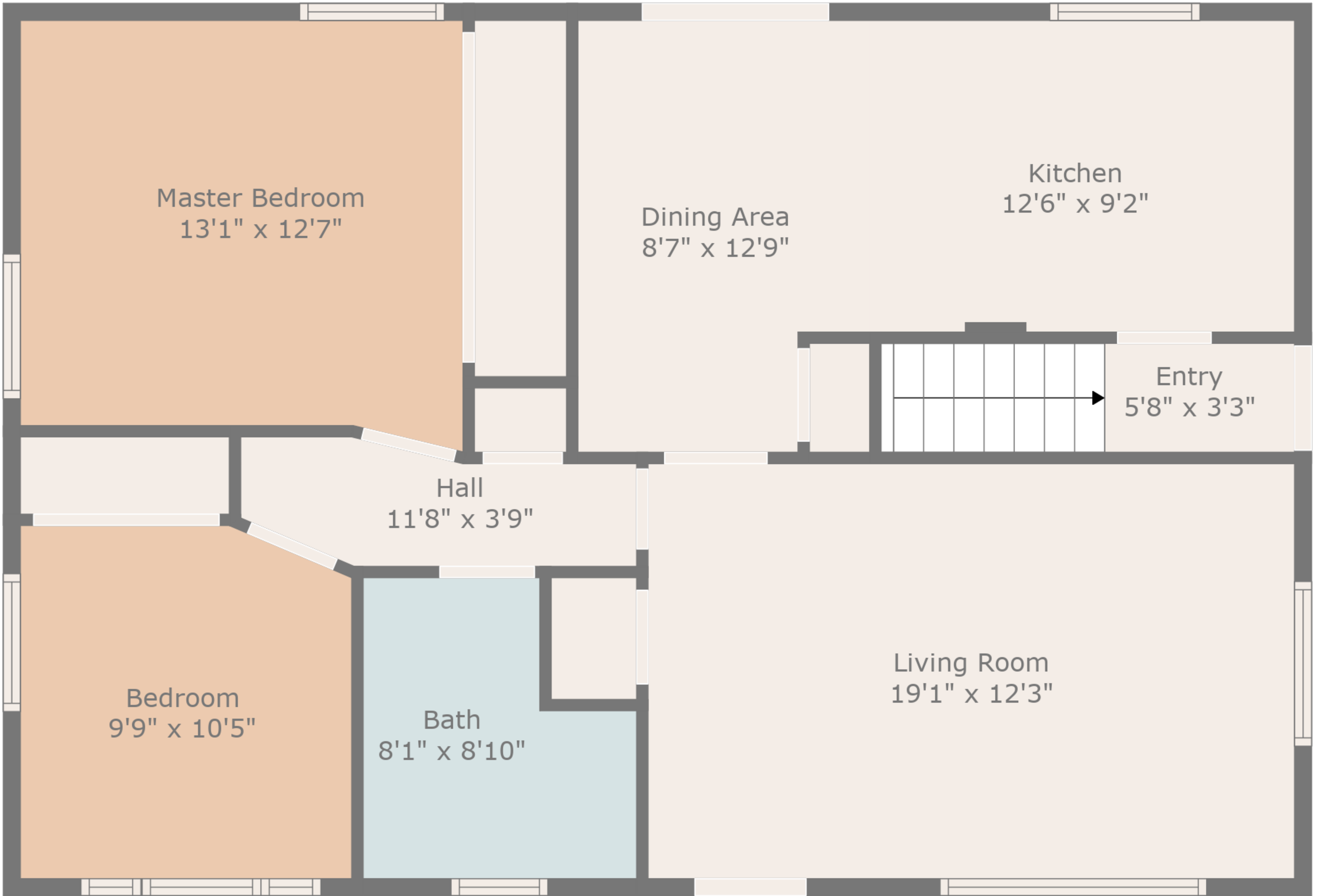
Floor 2
