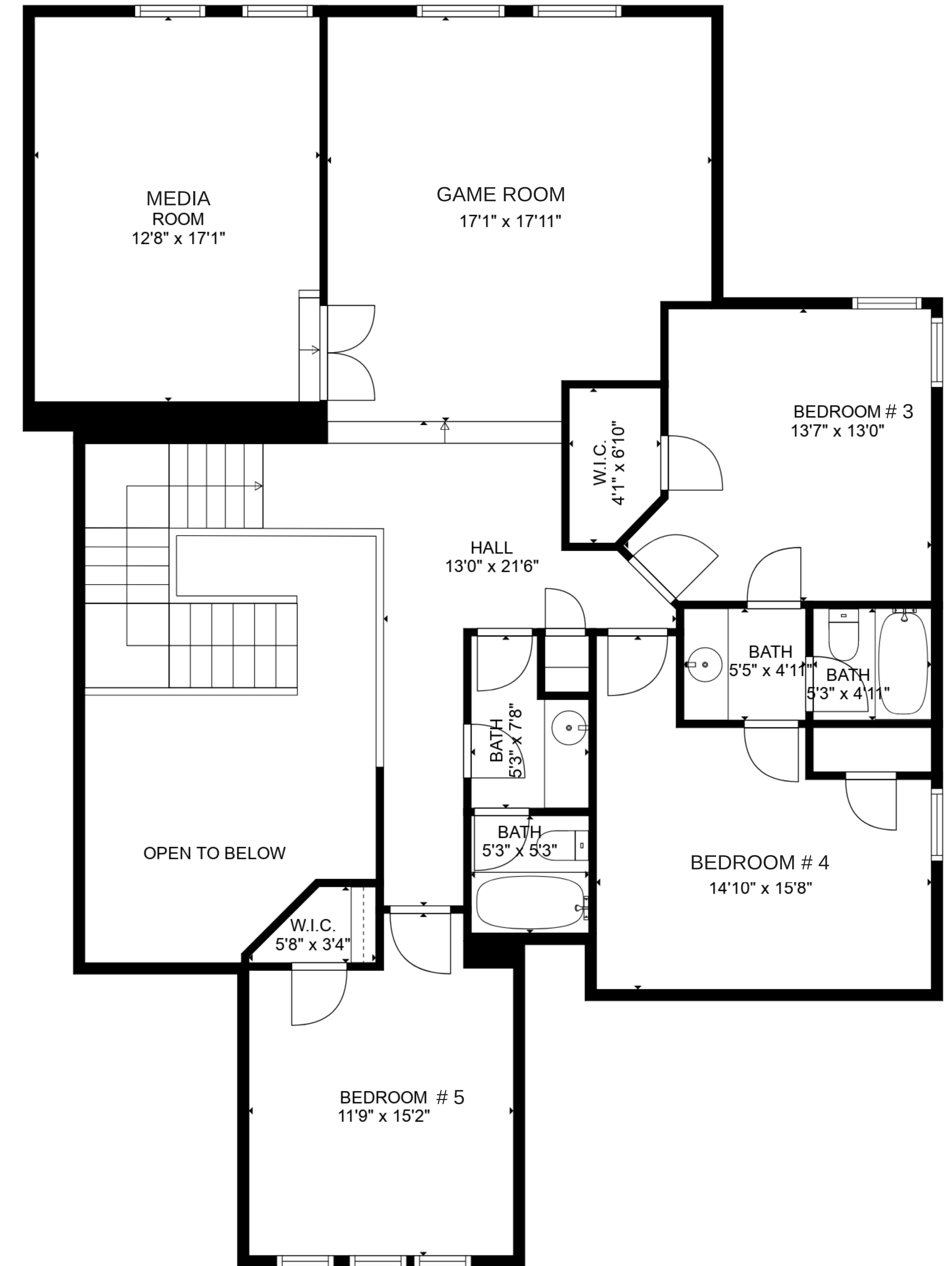
FLOOR 2
