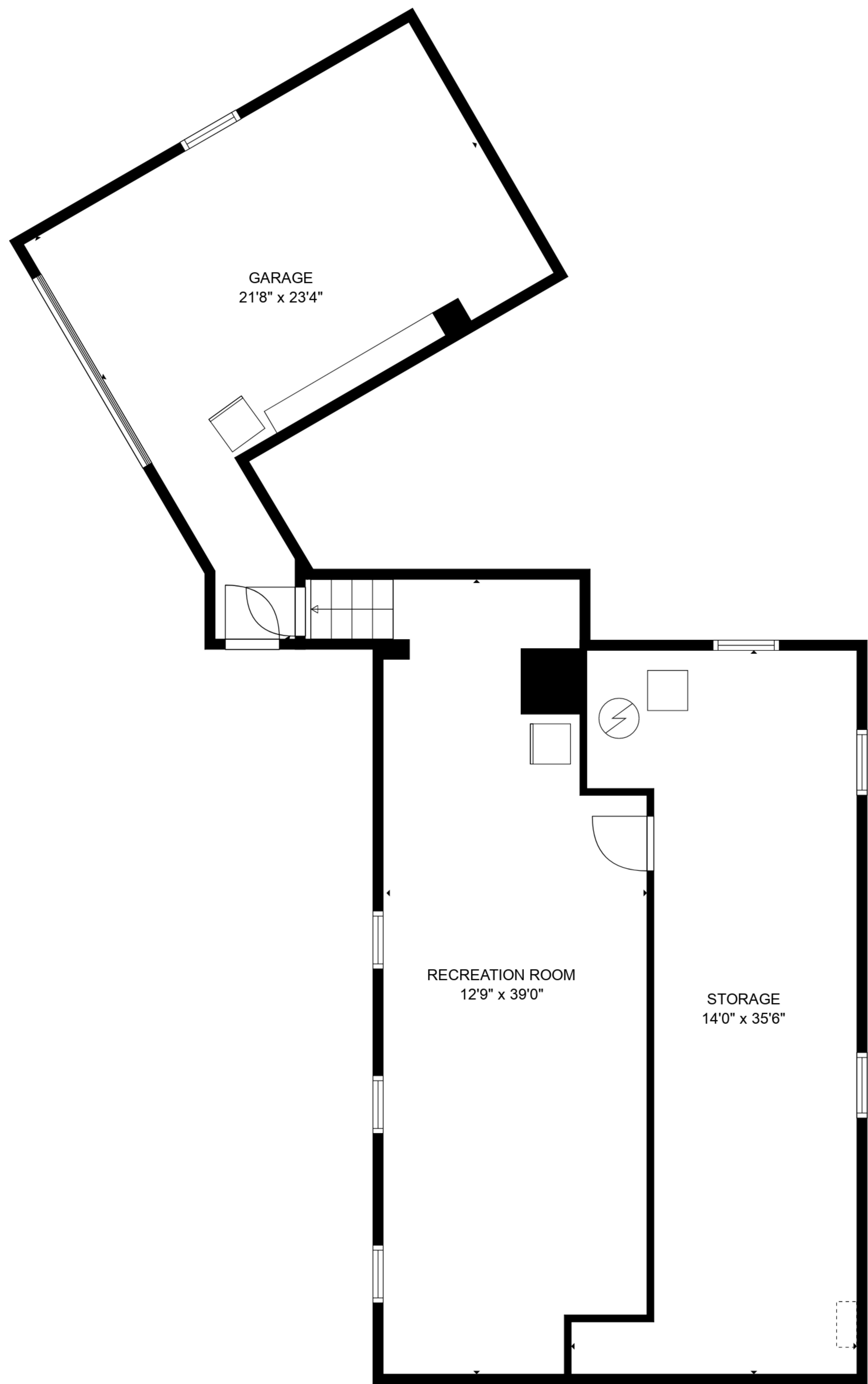
FLOOR 1
