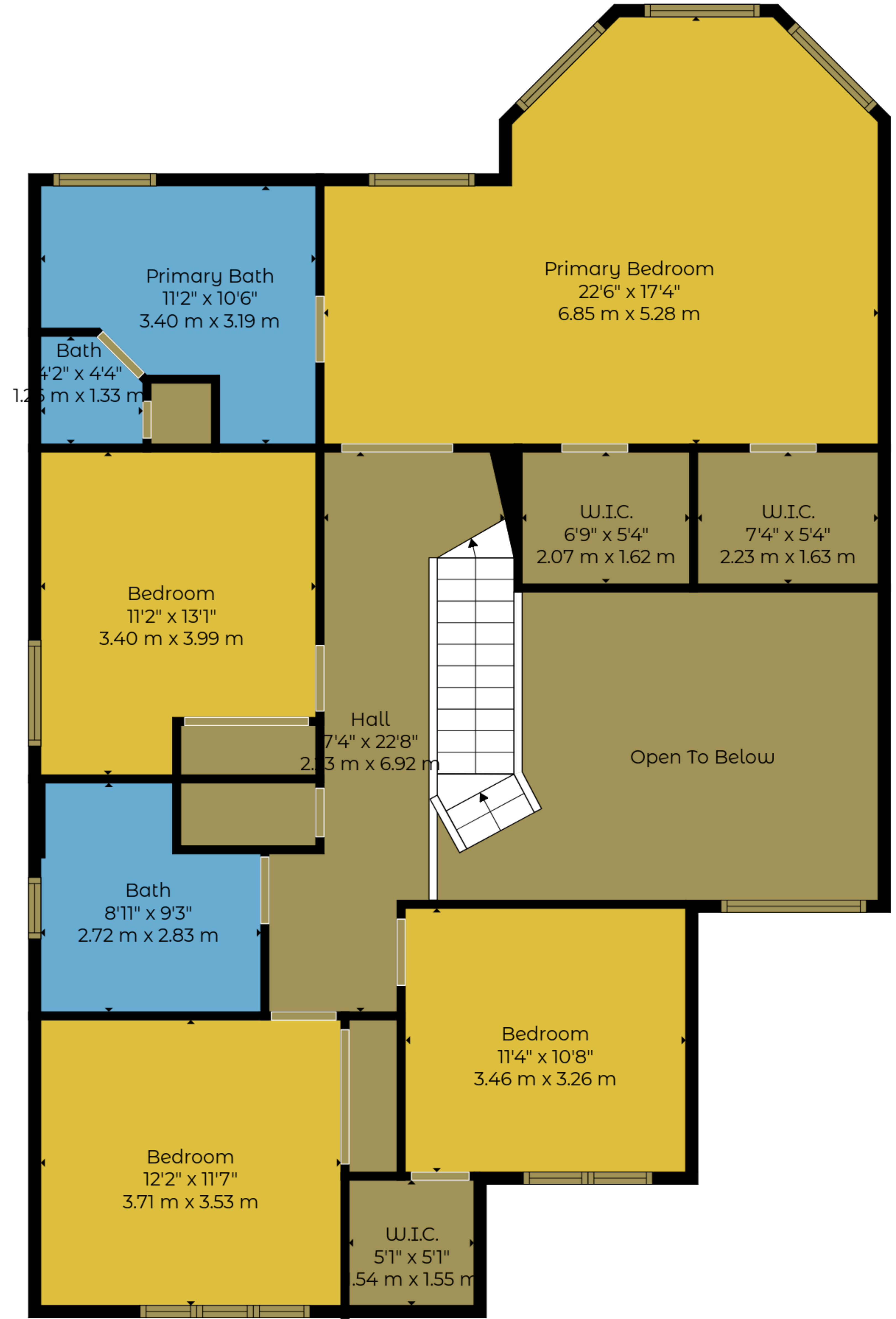
Floor 3
