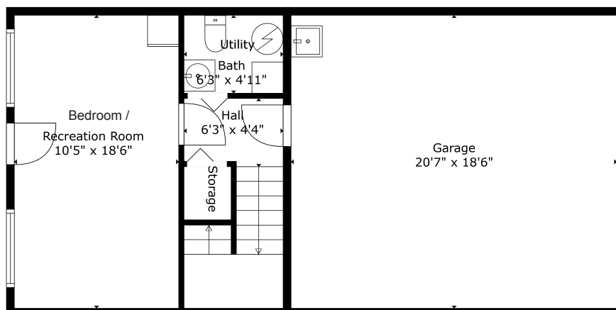
LOWER FLOOR 348 SQ.FT. CEILING HEIGHT 8'
