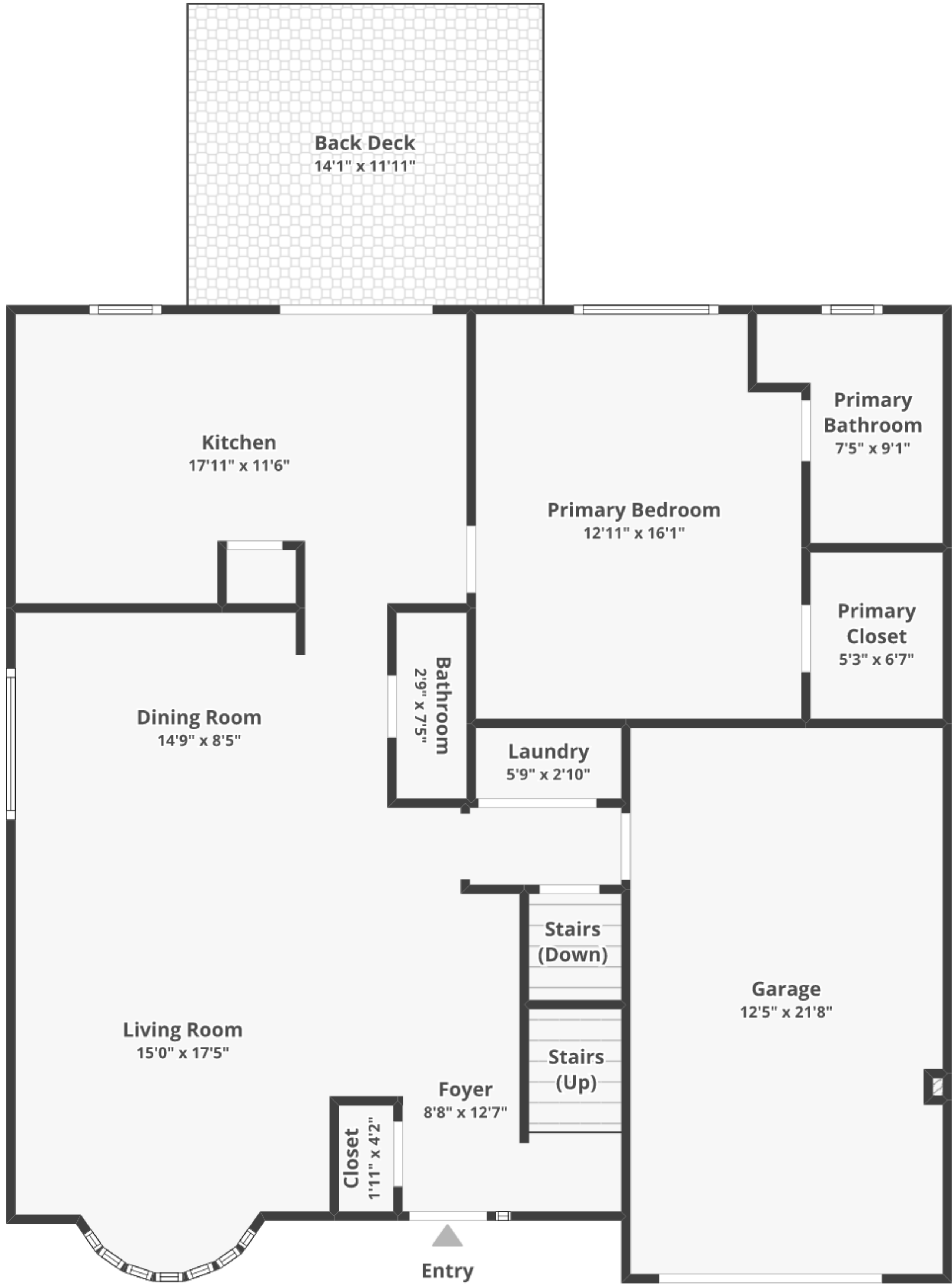
FLOOR 1
